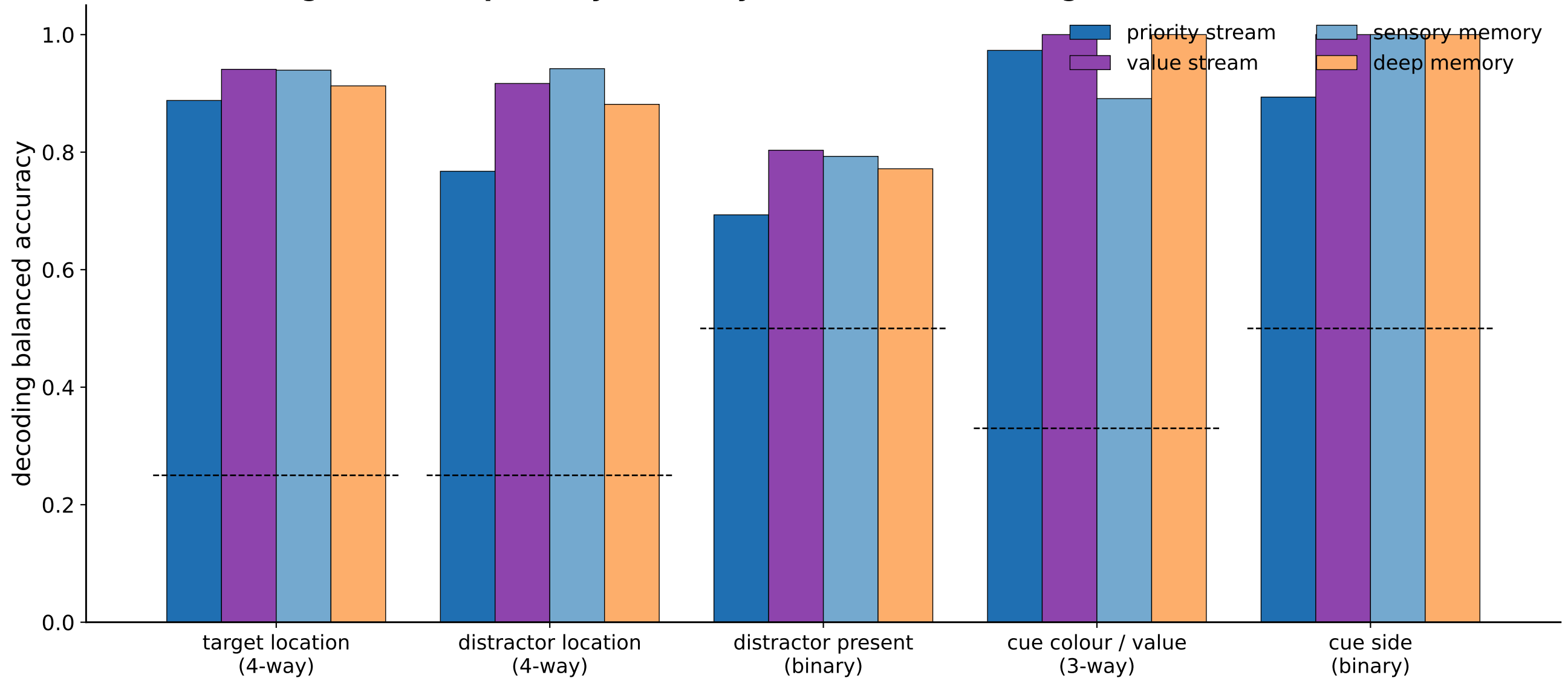
Linear decoding from each pathway / memory (2 frames after change)
