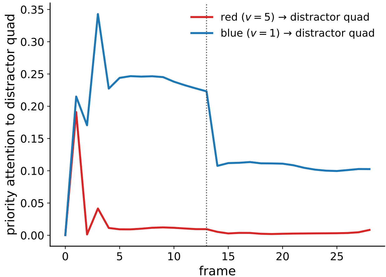
B Low value \rightarrow filter leaks onto distractor
