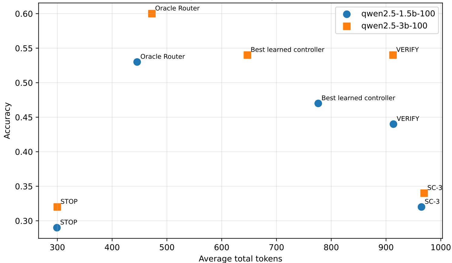
Model Comparison: Accuracy vs Token Cost
