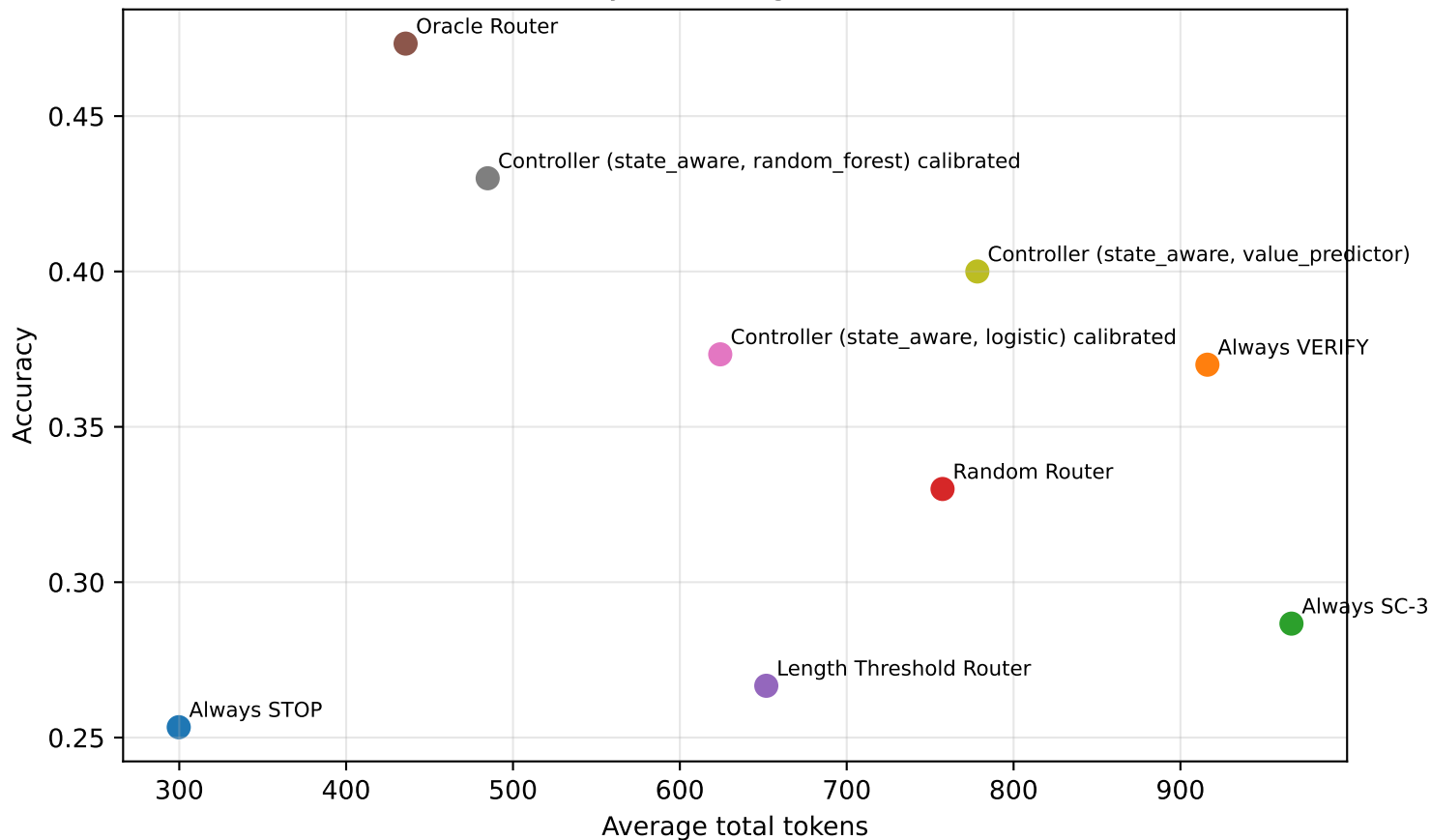
Accuracy vs Average Token Cost
