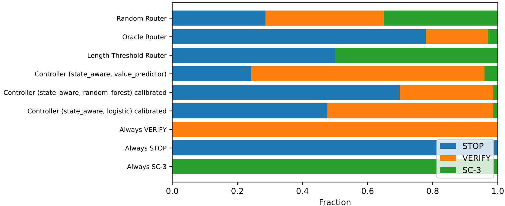
Action Distribution
