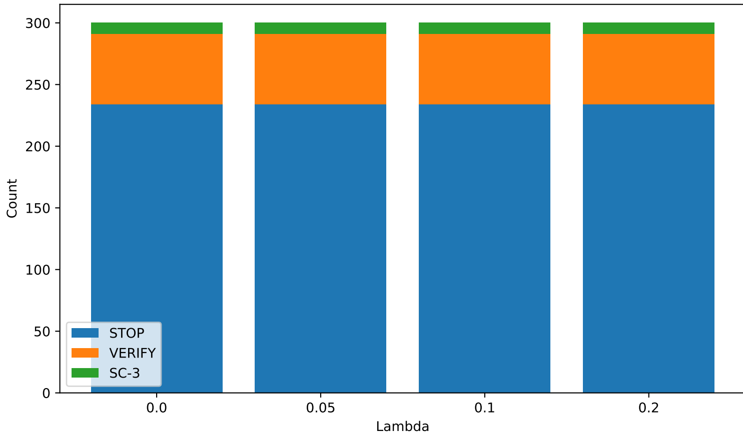
Oracle Action Distribution vs Lambda
