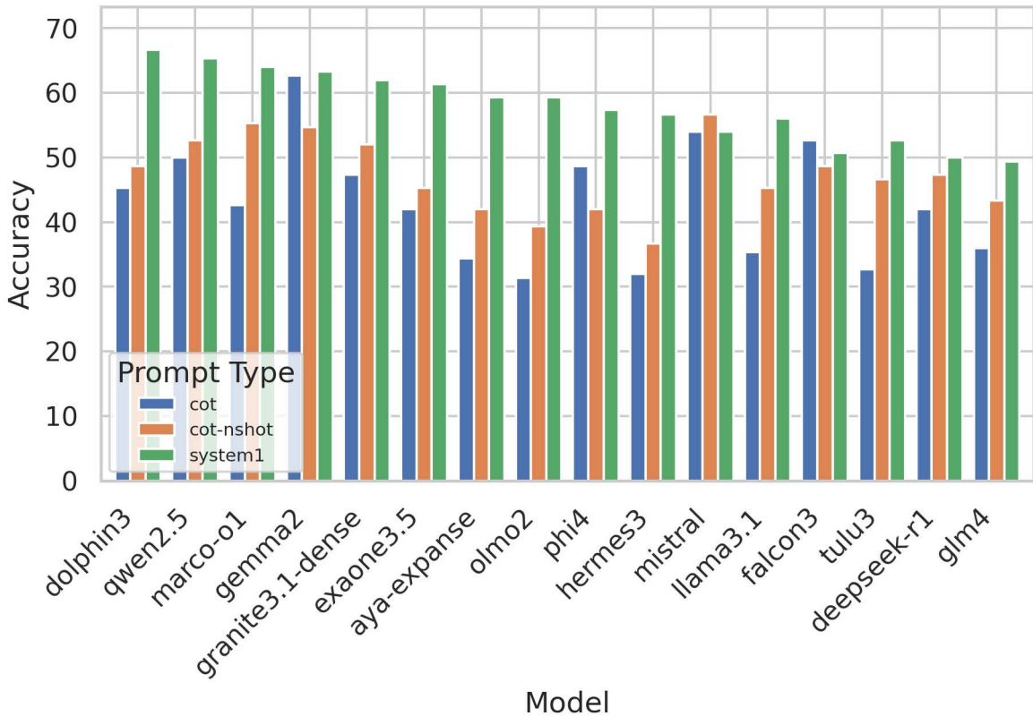
Accuracy by Model and Prompt Type (StandardLLM)
