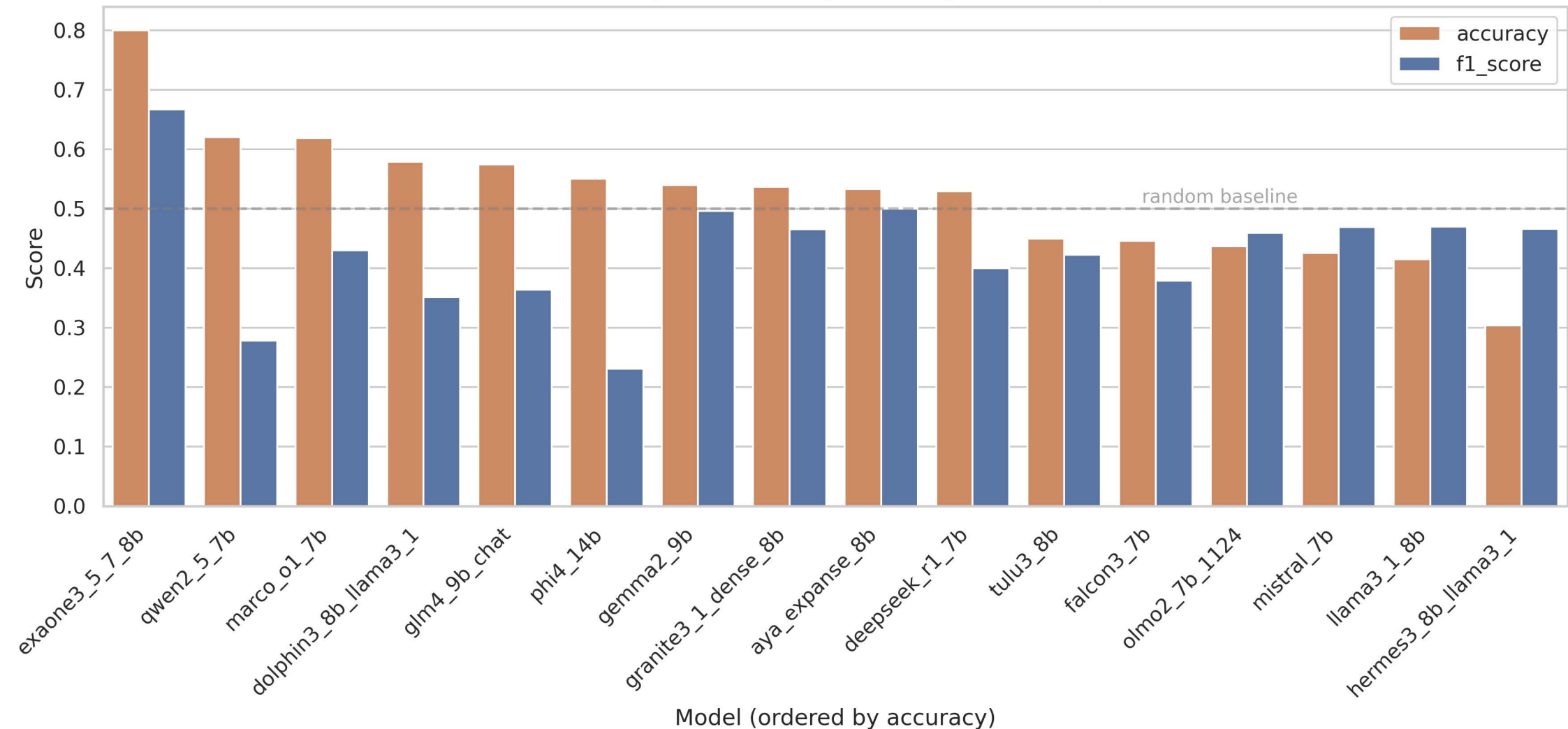
Accuracy vs F1-Score by Model (AgenticSimLLM)
