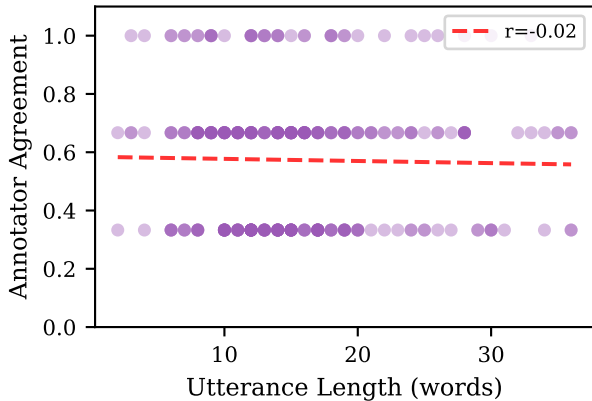
(b) Utterance Length vs Agreement
