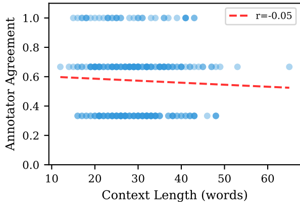
(a) Context Length vs Agreement
