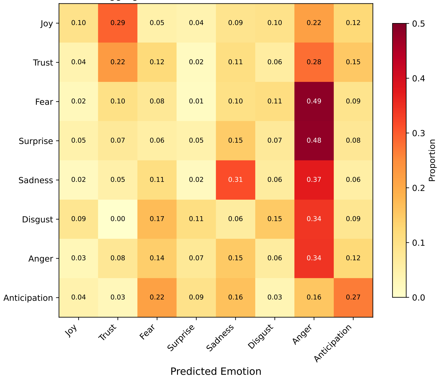
Model Prediction Confusion Matrix (aggregated across 7 models, row-normalized)
