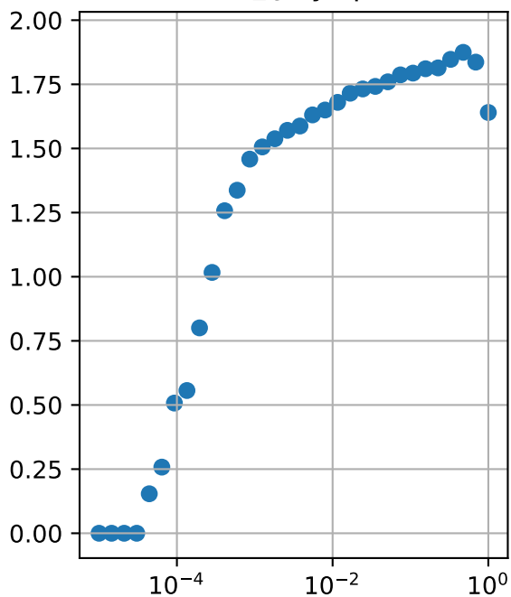
dim L_{\leq \varepsilon} by spore
