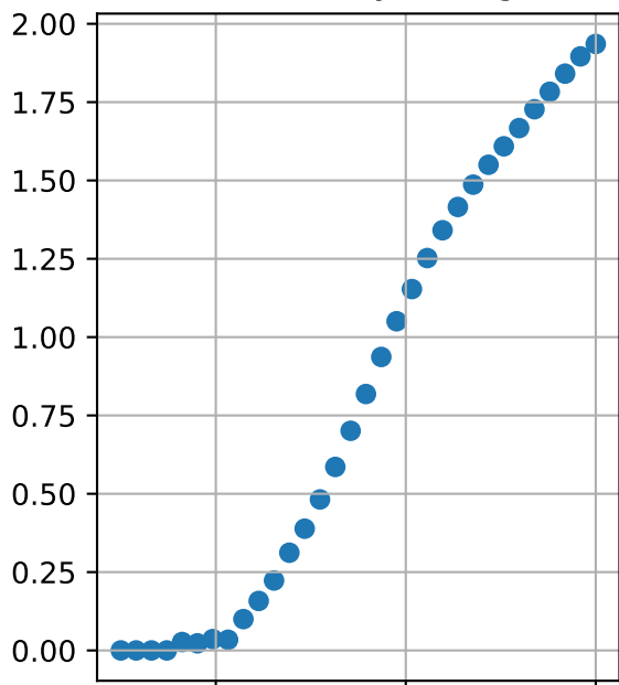
dim L_{\leq \varepsilon} by lin reg
