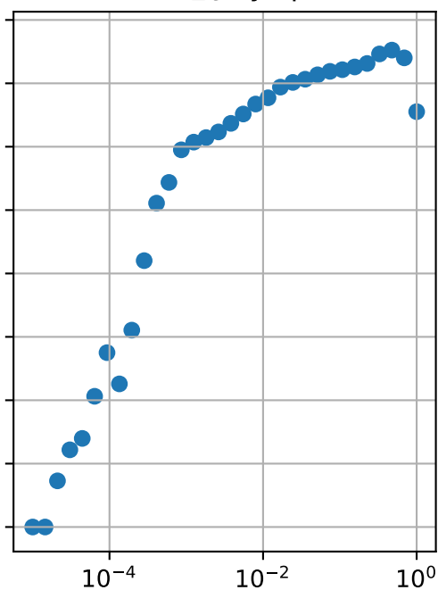
dim \partial L_{\leq \varepsilon} by spore
