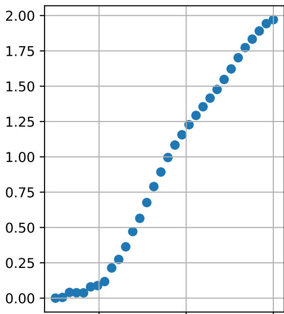
dim L_{\leq \varepsilon} by lin reg
