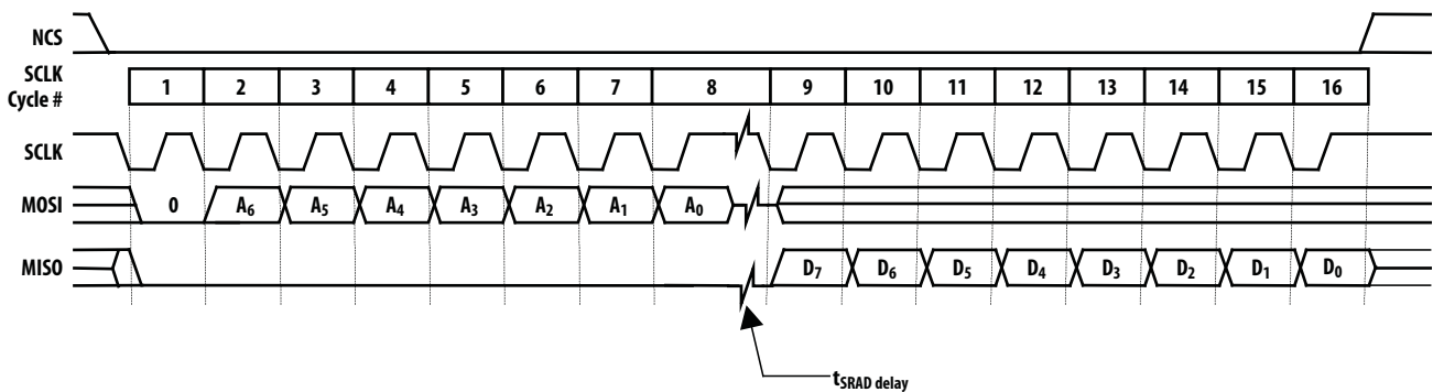
Figure 15. Read Operation
