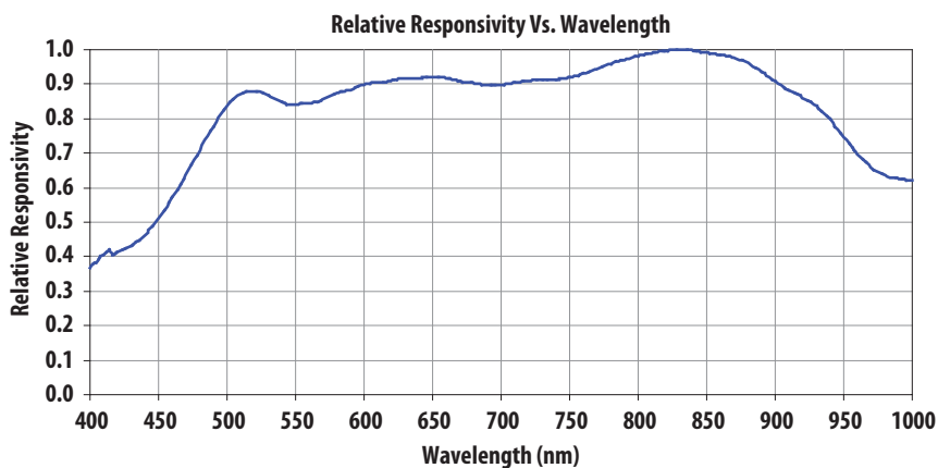
Figure 12. Wavelength Responsivity
