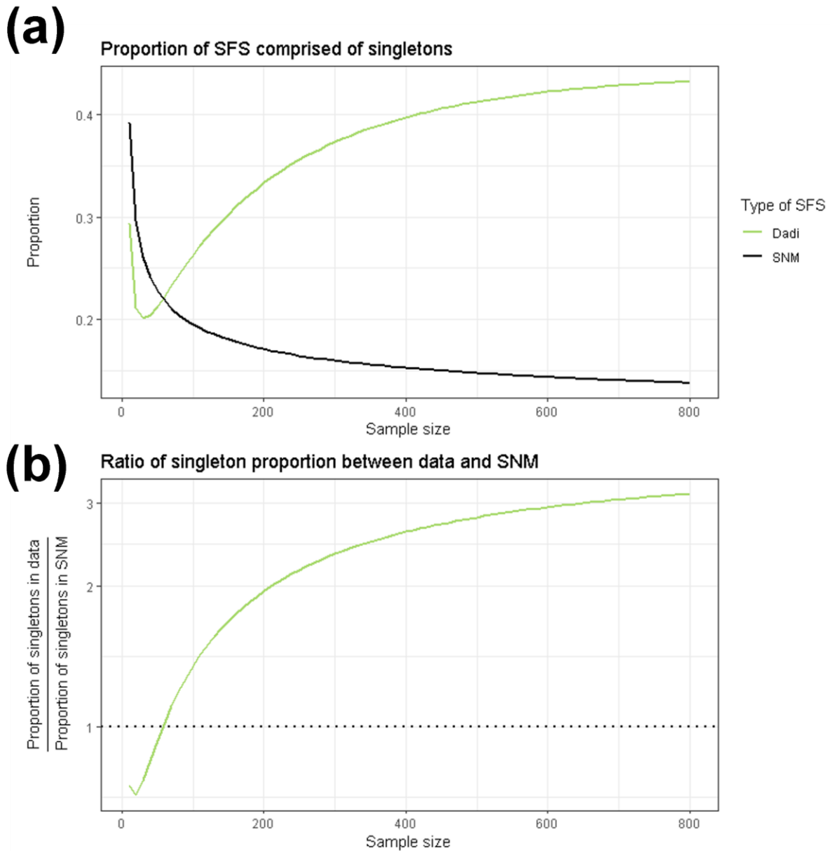
Figure S3: Proportion of SFS composed of singletons for SFS generated using \partial a \partial i .
