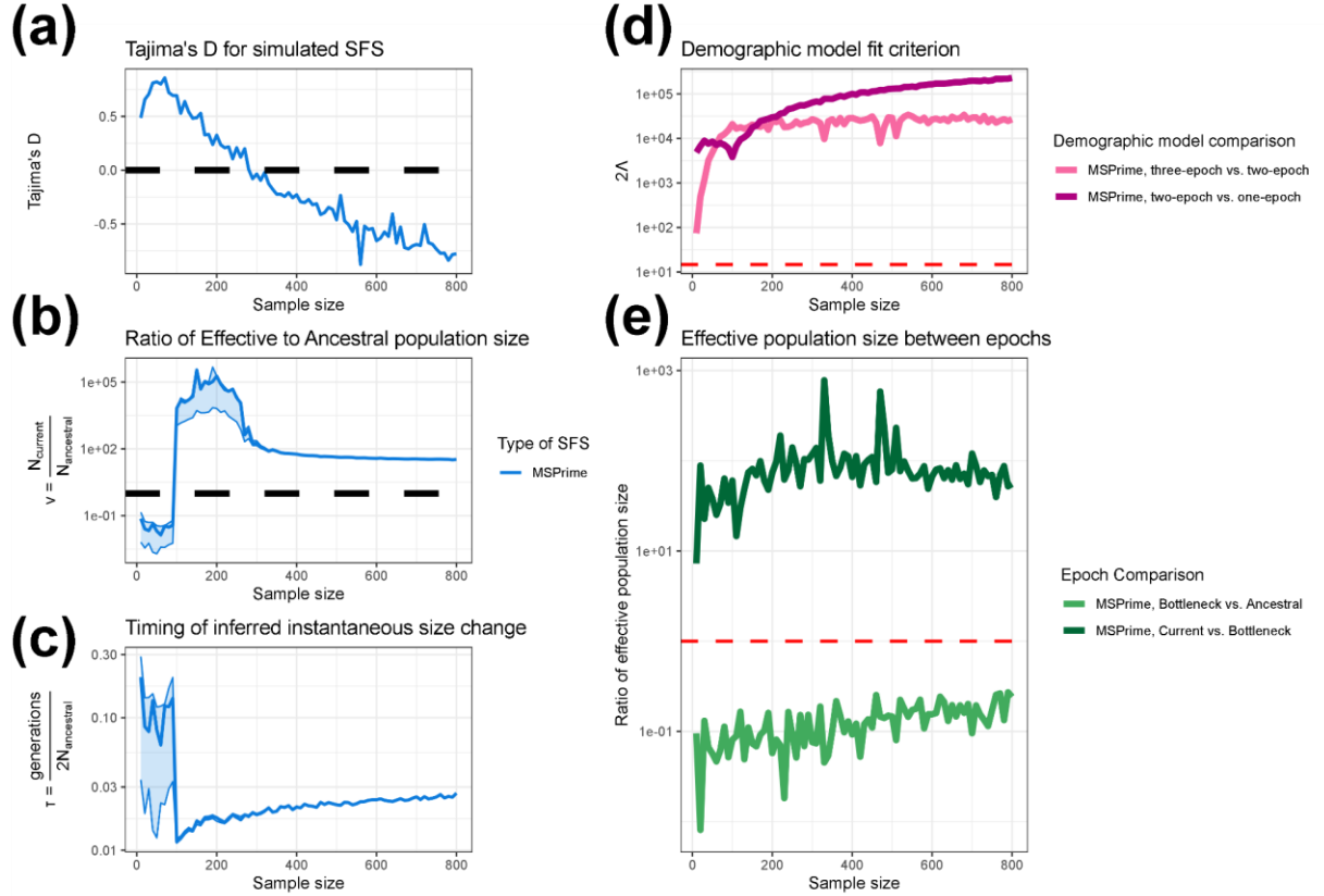
Figure 2. Demographic inference from data simulated under a three-epoch population history using MSPrime. a–c) Results from fitting a two-epoch demographic model to the simulated data across a range of sample sizes. a) Tajima's D for simulated SFS at different sample sizes. The dashed black line indicates a value of 0. b) The inferred effective population size change in units of N_{\text{Anc}} for a two-epoch model fit to the simulated data. The dashed black line indicates a value of 1. c) The estimated timing of the instantaneous size change for a two-epoch model in units of \frac{\text{generations}}{2N_{\text{Anc}}} . Lightly shaded areas indicate the approximate 95% confidence interval for v and \tau , corresponding to parameter values with a log likelihood less than three units from the MLE. d) The likelihood ratio test statistic, 2\Delta , comparing the fit of one-, two-, and three-epoch demographic models. The dashed red line indicates a critical value of 14.76. e) The ratio of inferred effective population size between epochs when fitting a three-epoch demographic model (the correctly specified model) to the simulated data. Bottleneck vs. ancestral compares the ratio of inferred population size in the bottleneck epoch to the ancestral population size. The fact that it is less than 1 for all sample sizes indicates that, going forward in time, we correctly infer an initial population contraction. Recent vs. bottleneck compares the ratio of inferred population size in the current (i.e. most recent) epoch to that in the bottleneck epoch. The fact that it is >1 for all sample sizes indicates that, going forward in time, we correctly infer a recent population expansion. The dashed red line indicates a size change ratio of 1 between epochs. The x-axis for all figures indicates the numbers of individuals analyzed in the dataset.
