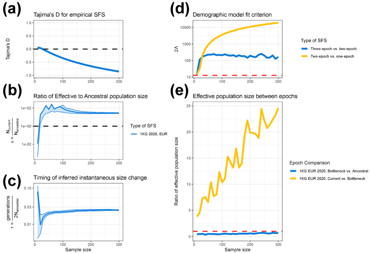
Figure 6. Analysis of empirical 1000 Genomes EUR data shows how demographic inference behaves as a function of the number of individuals analyzed. We applied a similar inference pipeline to high quality empirical data from humans of European descent (Auton et al. 2015; Byrska-Bishop et al. 2022) (see Methods), fitting one-, two-, and three-epoch demographic models at varying sample sizes to examine how demographic parameters change. In all figures, the x-axis shows the sample size used in demographic inference. The y-axis shows the inferred effective population size change in units of N_{Anc} for a two-epoch model (a), the estimated timing of the instantaneous size change for a two-epoch model in units of \frac{generations}{2N_{Anc}} (b), Tajima's D (c), the model comparison statistic 2\Lambda (d), which compares the fit of three-epoch and two-epoch models, and the ratio of inferred effective population size between epochs in a three-epoch demographic model (e). Lightly shaded areas indicate the approximate 95% confidence interval for v and \tau , corresponding to a log likelihood three less than the MLE (a-b). The dashed red line in Figure 6D indicates a critical value of 12.79. On the right-hand side the x-axis denotes the population size change parameter, v , and the y-axis shows the time parameter, \tau .
