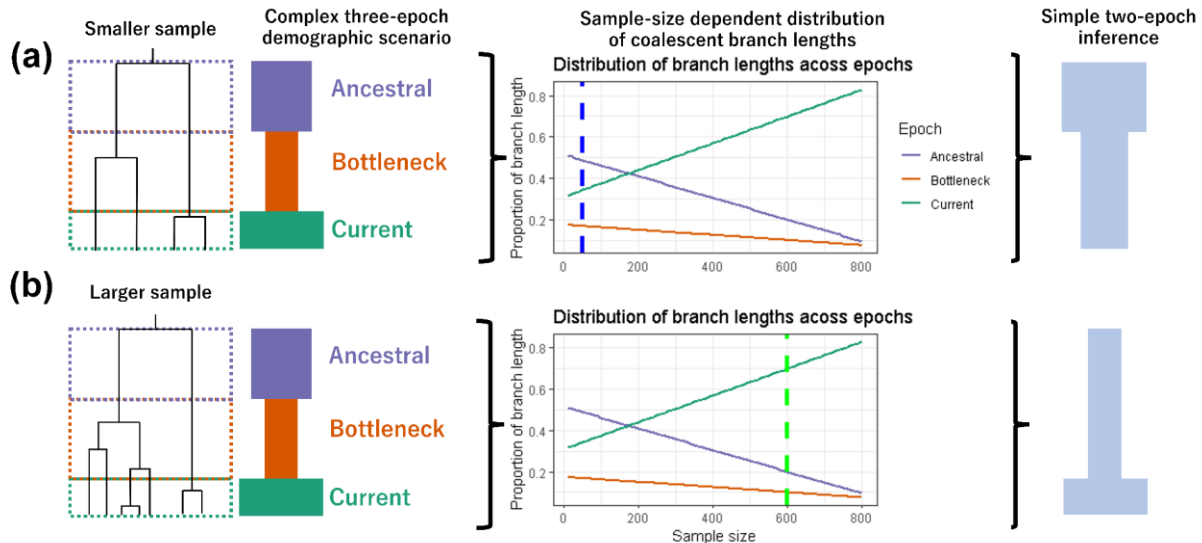
Figure 4. Schematic depicting effects of sample size on branch lengths and inferred two-epoch demography. (a) A simulated three-epoch demographic scenario consisting of an ancestral epoch, a bottleneck epoch, and the current epoch. Branch lengths on the coalescent tree are partitioned according to the epoch in which they occur. In this example, the largest proportion of coalescent branch lengths falls within the ancestral epoch. Consequently, when fitting a simplified two-epoch model to this data, we would expect to infer a population contraction. (b) The same three-epoch demographic scenario with a larger sample size. The increased number of sampled lineages alters the distribution of branch lengths across epochs, and as a result the largest proportion of coalescent branch lengths now falls within the current epoch. Consequently, fitting a simplified two-epoch demographic model yields a qualitatively different demographic scenario despite the underlying simulated history being identical.
