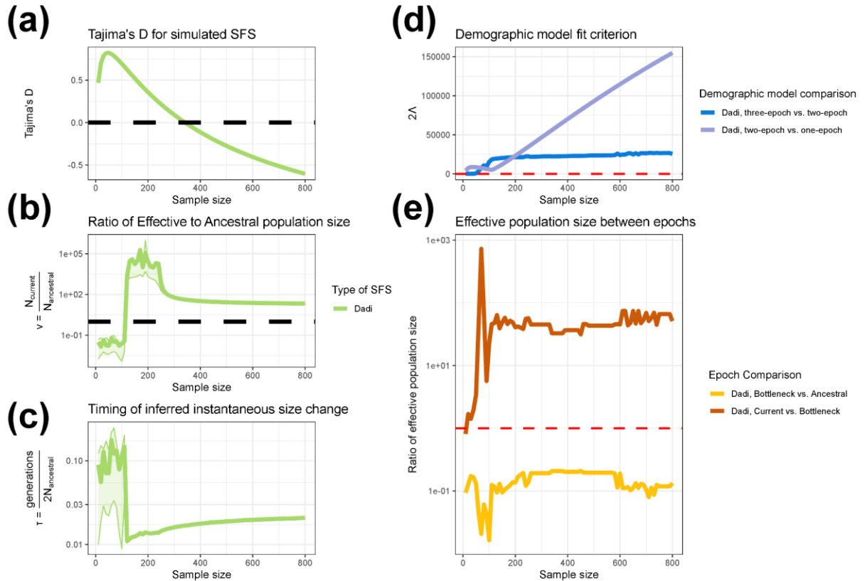
Figure S2: Demographic inference for SFS generated using \partial a \partial i
