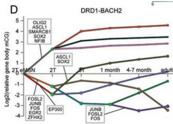
Figure 3: DREM model fit for the DRD1-BACH2 trajectory using the regenerated TF-DMR prior. Developmental stages advance left-to-right across the lineage. Split nodes are annotated with the transcription factors whose targets are significantly enriched, by DREM's hypergeometric test, among the genes assigned to an outgoing path relative to the genes entering the split.
