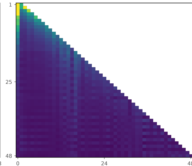
Sliced LR-AttnRes Full r=256
