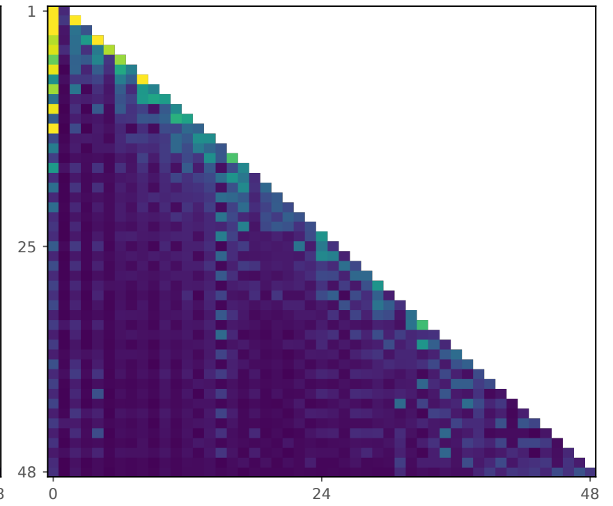
Sliced LR-AttnRes Full r=512
