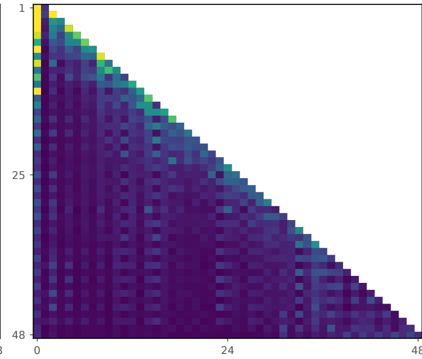
Sliced LR-AttnRes Full r=256
