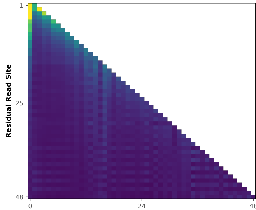
Sliced LR-AttnRes Full r=128
