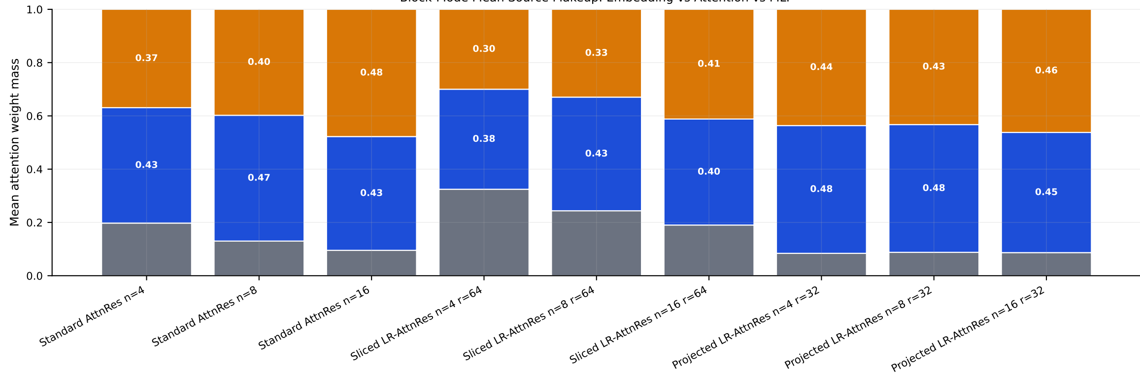
Block-Mode Mean Source Makeup: Embedding vs Attention vs MLP
