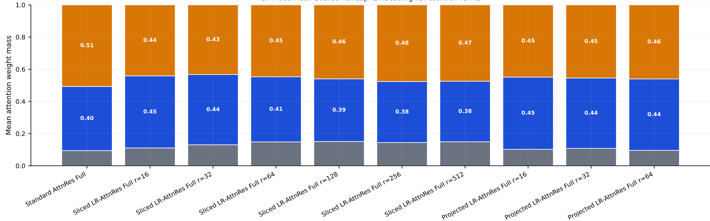
Full-Mode Mean Source Makeup: Embedding vs Attention vs MLP
