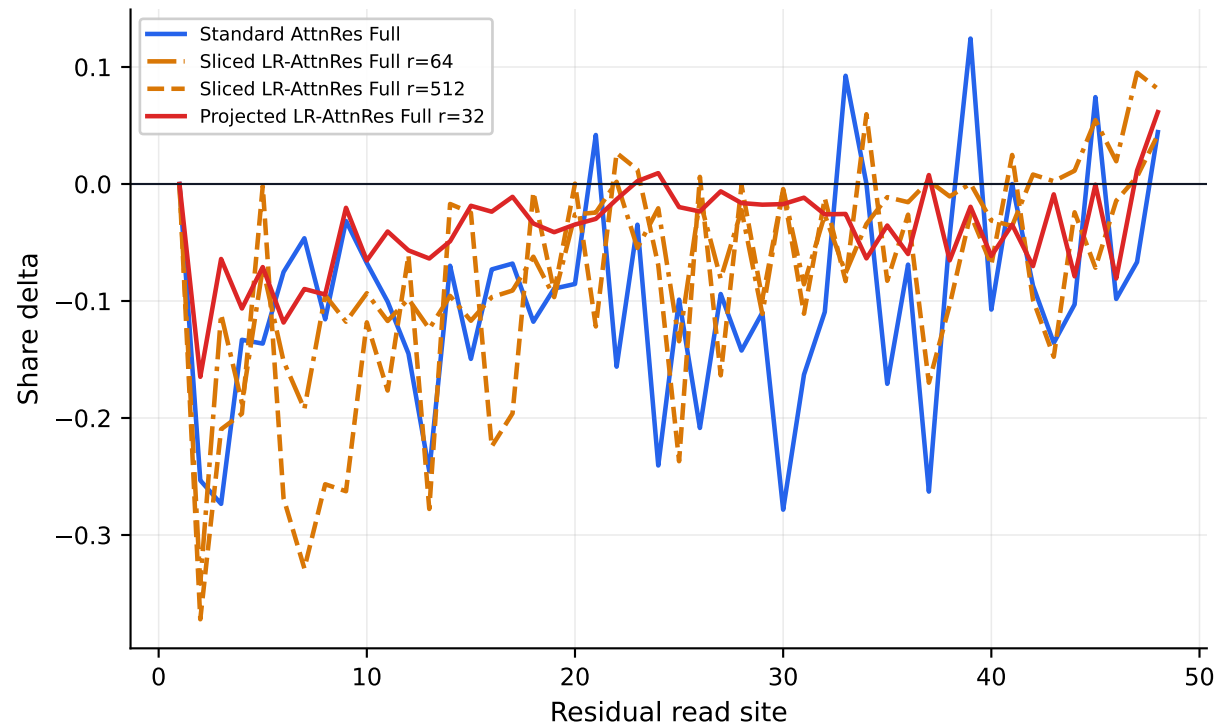
Observed Attn Share minus Count-Implied Share
