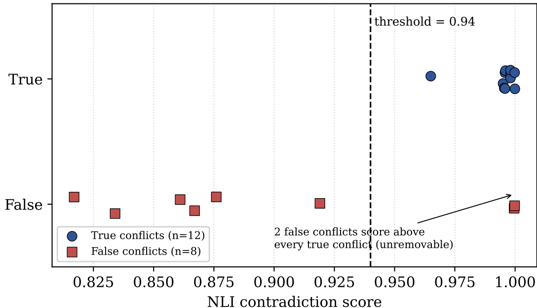
NLI score separation: true vs. false conflicts
