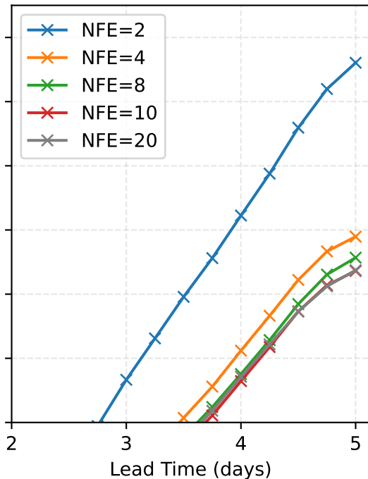
Warm Flow Matching (Ours)
