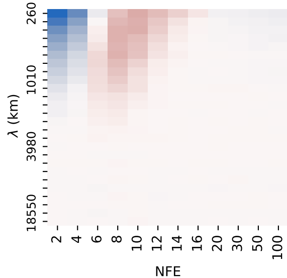
DPM Solver
