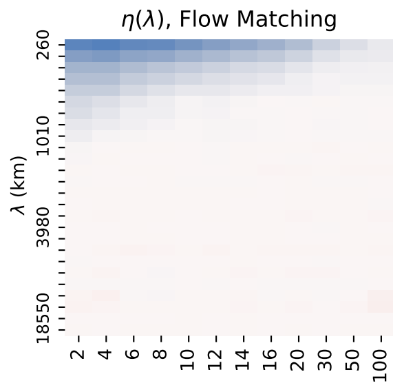
Midpoint Solver
