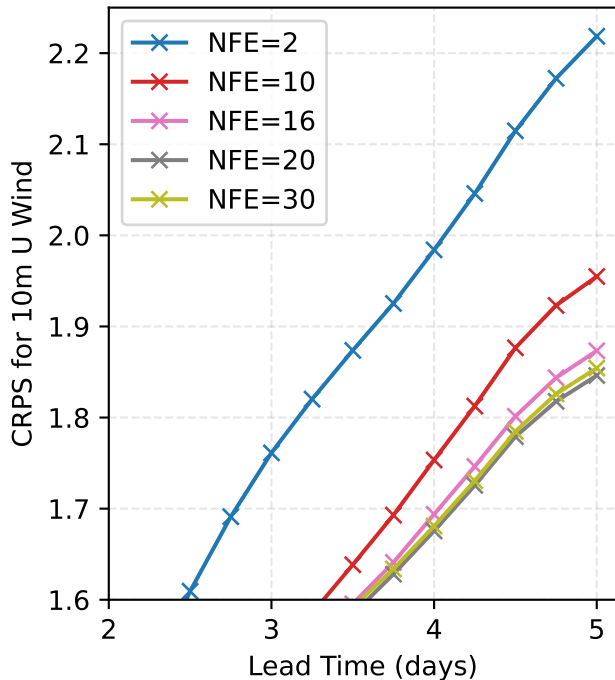
Flow Matching + DPM Solver
