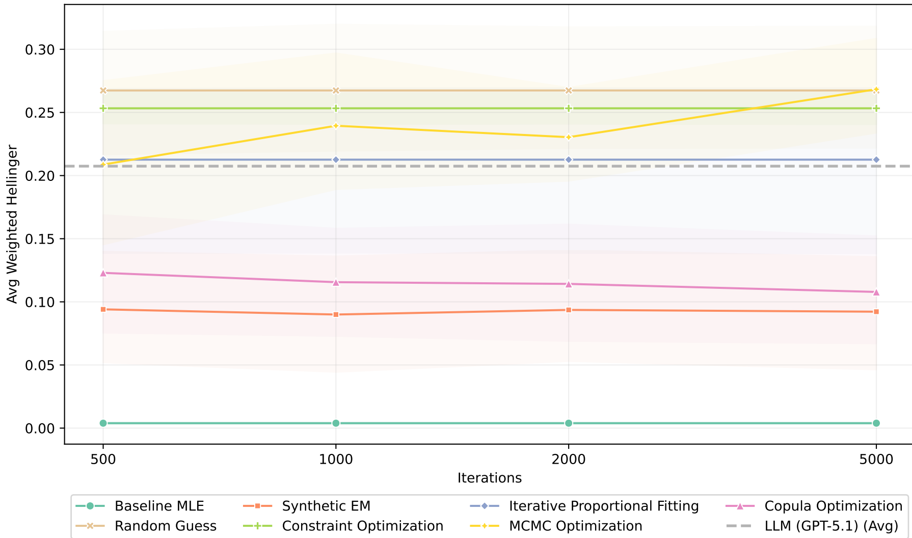
Global Convergence: Weighted Hellinger Distance
