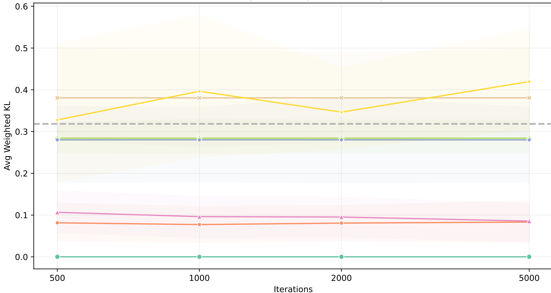
Global Convergence: Weighted KL Divergence
