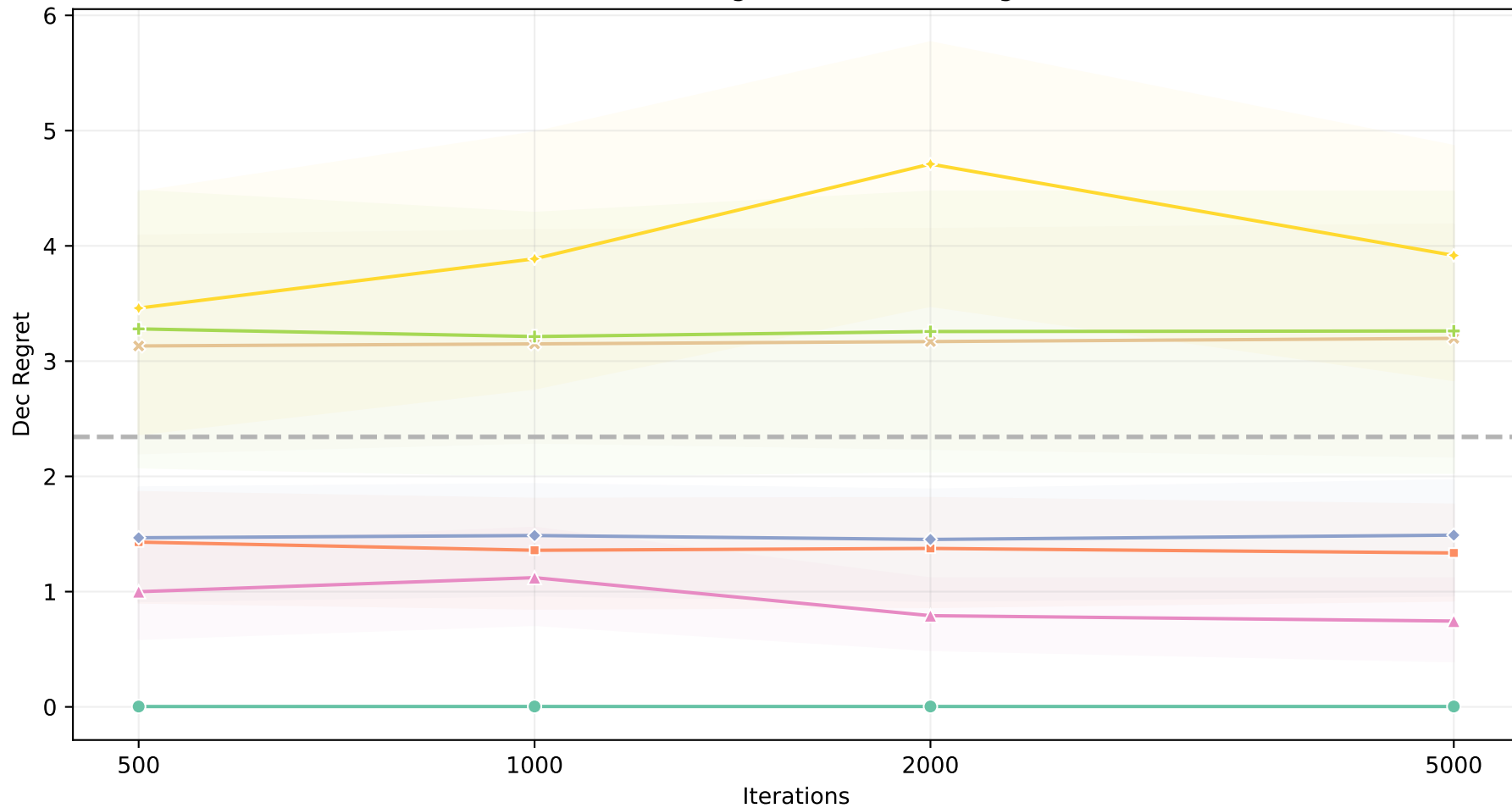
Global Convergence: Decision Regret
