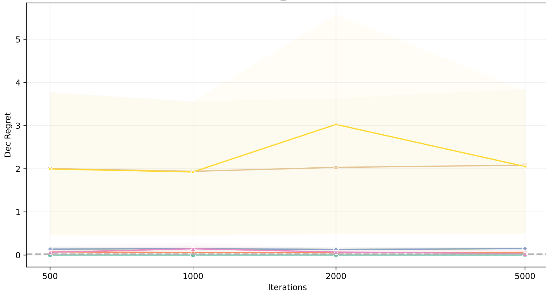
Convergence (binary_only): Decision Regret
