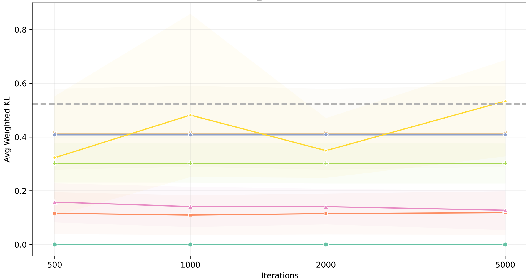
Convergence (discrete_only): Weighted KL Divergence
