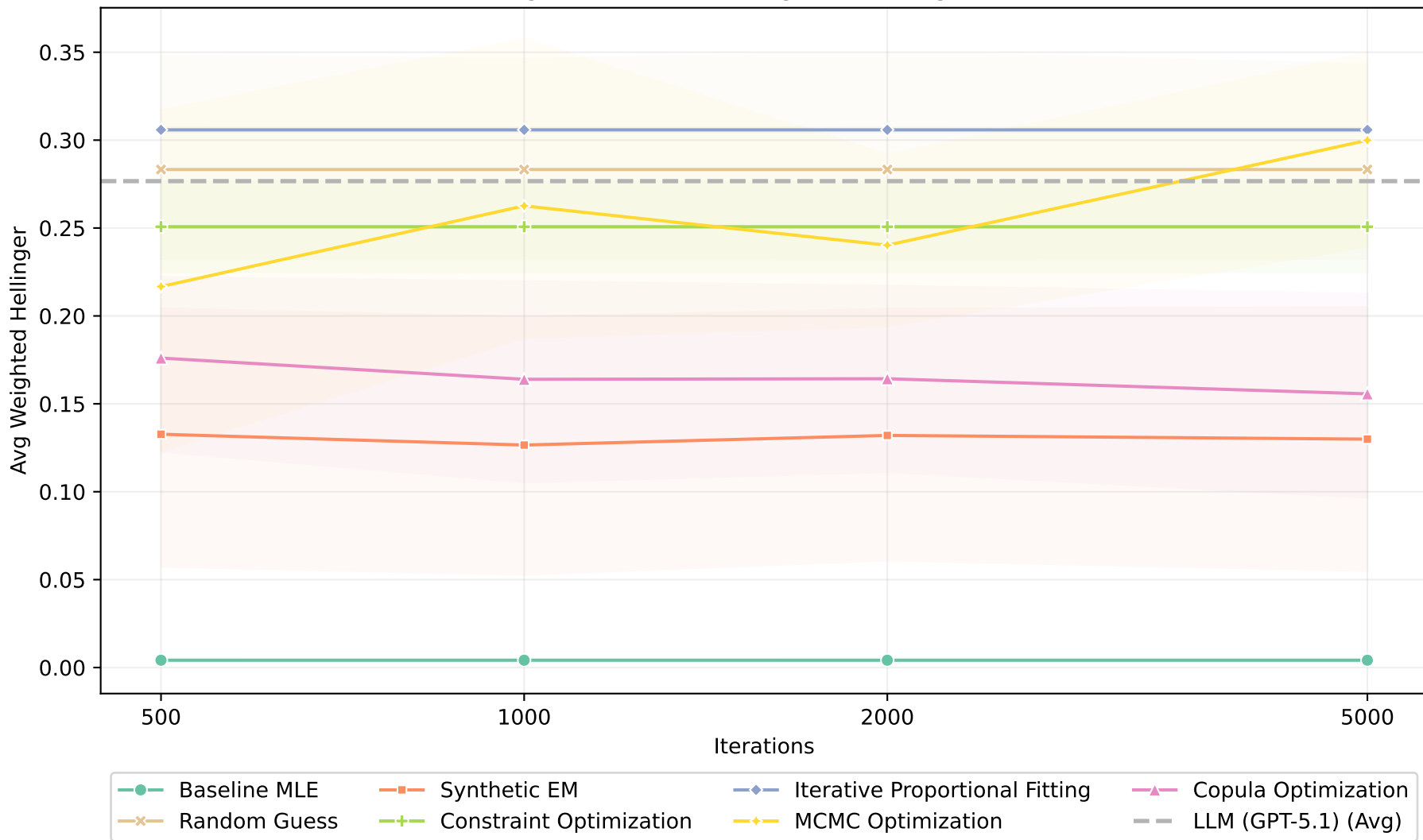
Convergence (mixed): Weighted Hellinger Distance
