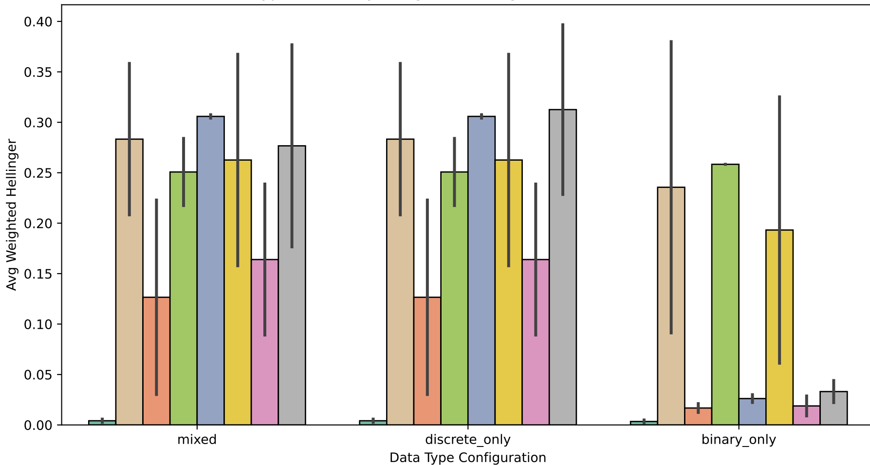
Data Type Sensitivity: Weighted Hellinger Distance (at 1000 iters)
