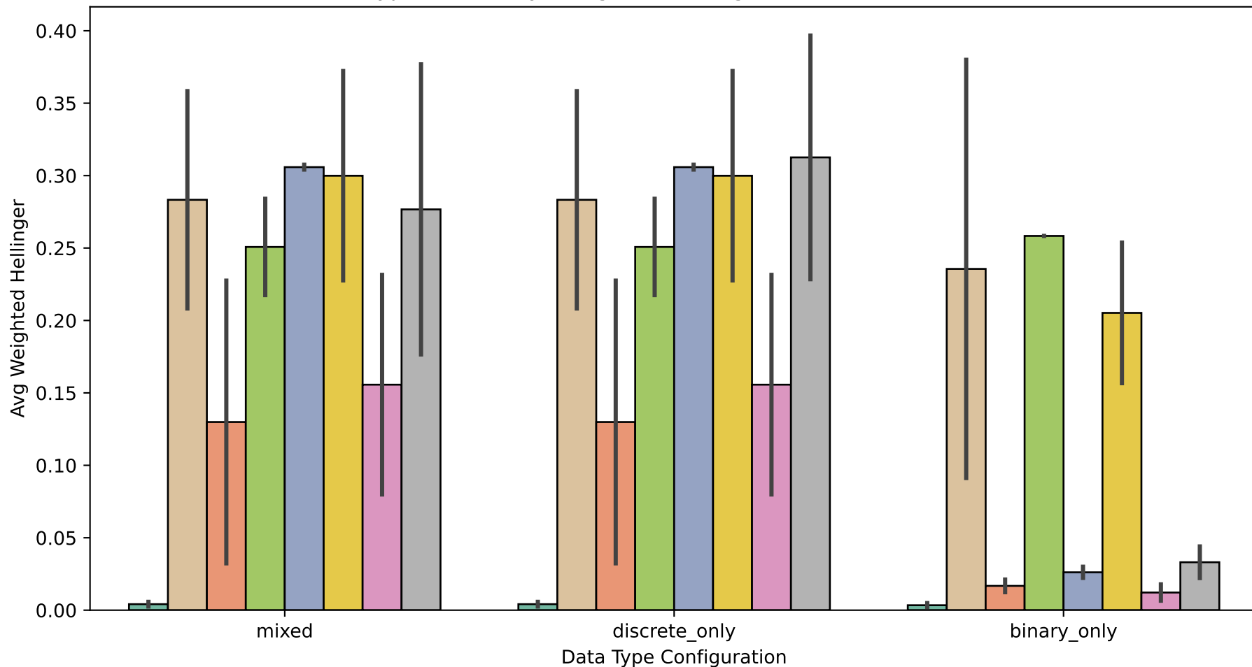
Data Type Sensitivity: Weighted Hellinger Distance (at 5000 iters)
