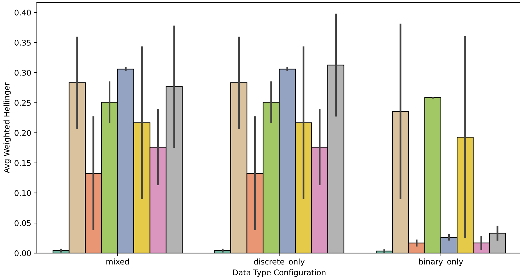
Data Type Sensitivity: Weighted Hellinger Distance (at 500 iters)
