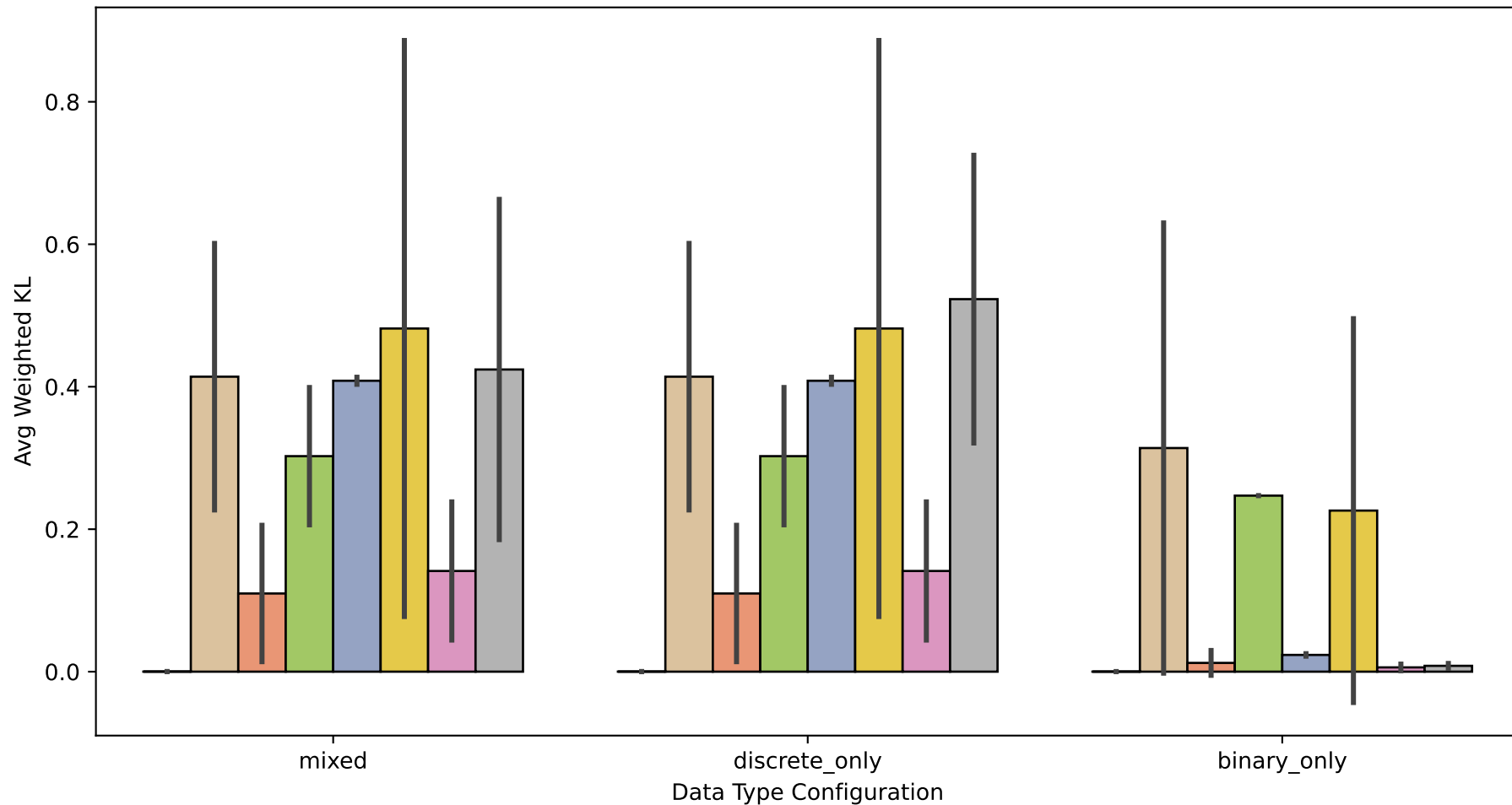
Data Type Sensitivity: Weighted KL Divergence (at 1000 iters)
