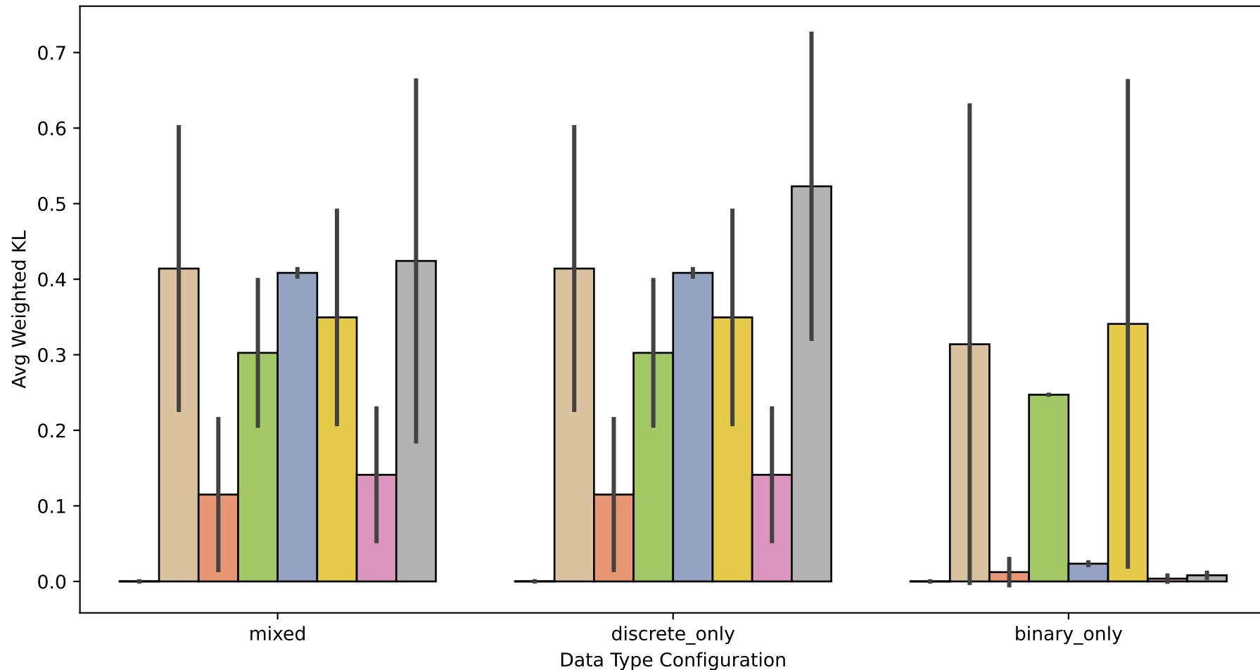
Data Type Sensitivity: Weighted KL Divergence (at 2000 iters)
