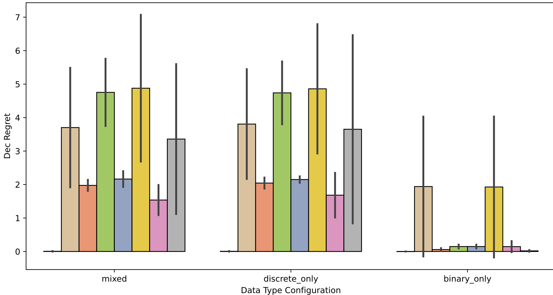
Data Type Sensitivity: Decision Regret (at 1000 iters)
