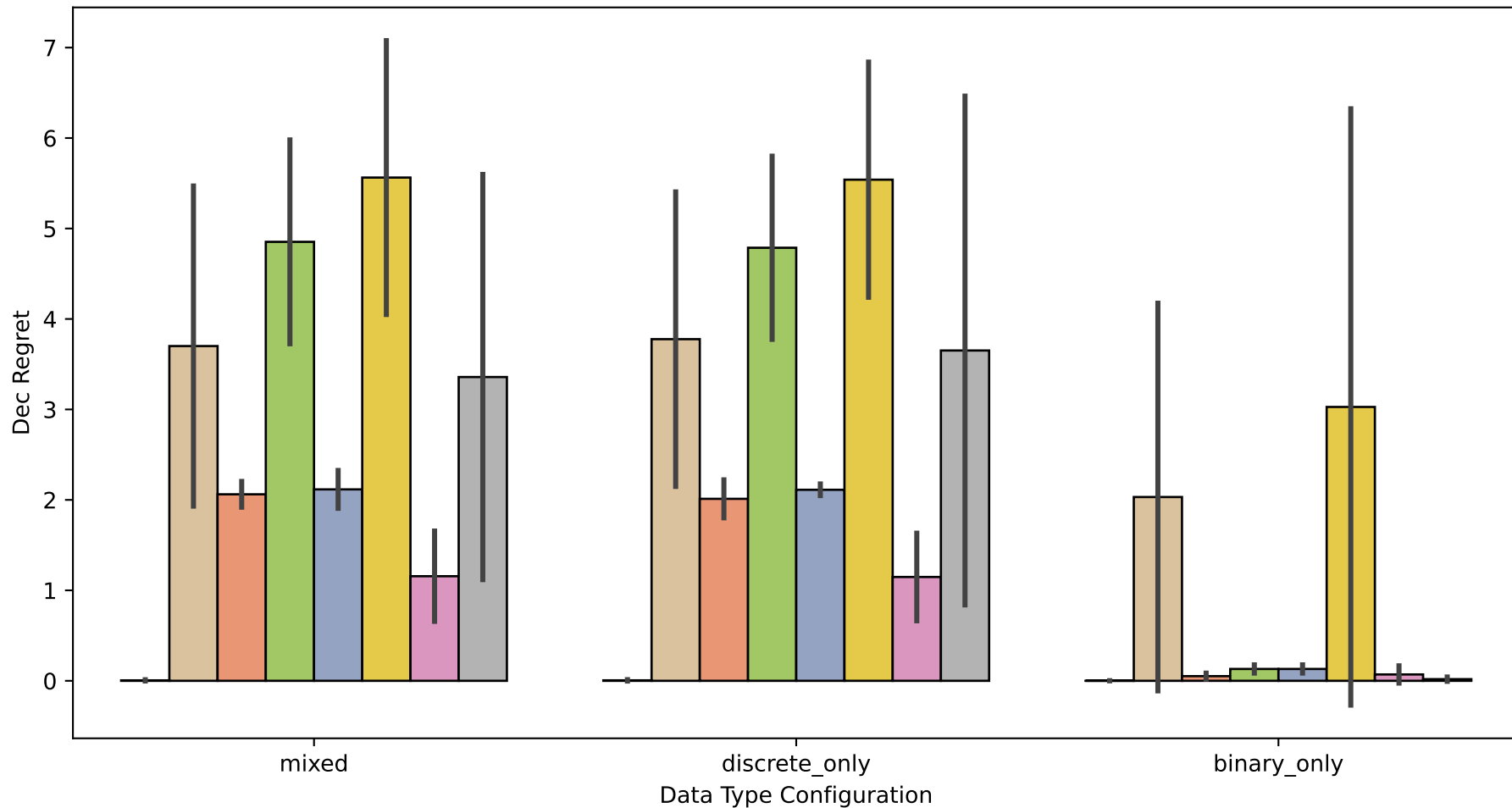
Data Type Sensitivity: Decision Regret (at 2000 iters)
