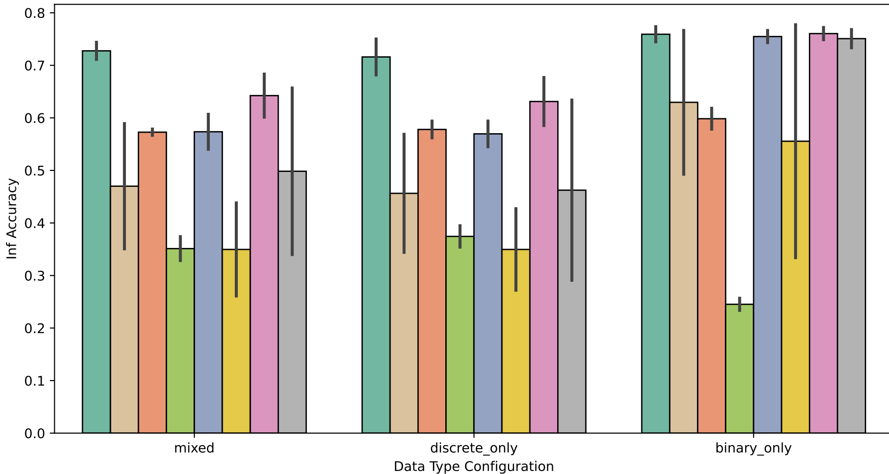
Data Type Sensitivity: Inference Accuracy (at 2000 iters)
