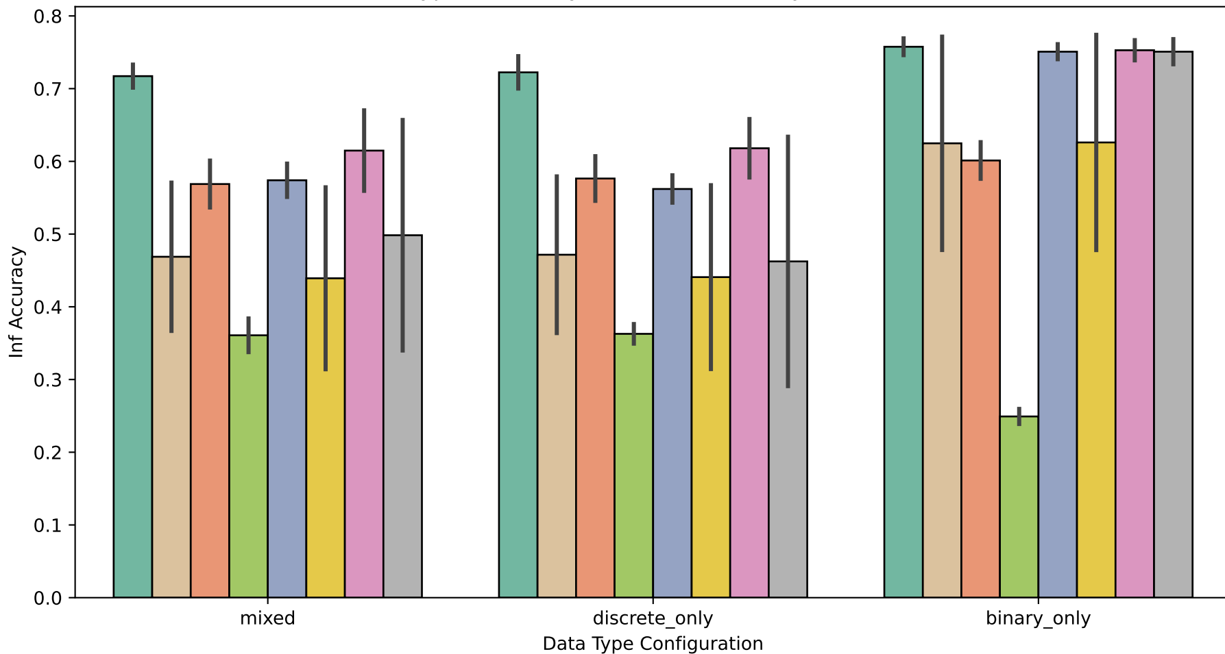
Data Type Sensitivity: Inference Accuracy (at 500 iters)
