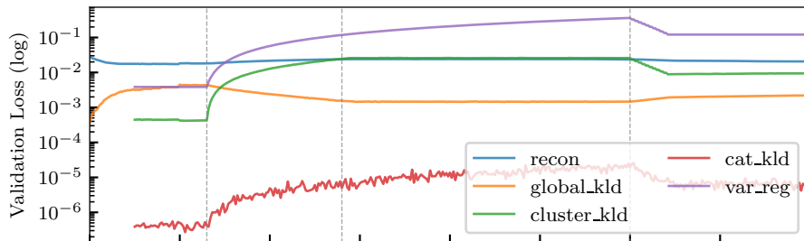
Validation Losses
