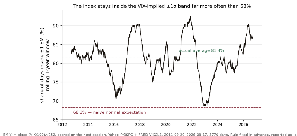
Figure 4. Rolling one-year share of sessions whose absolute next-day move stayed inside the VIX-implied \pm 1\sigma expected move, on 3,770 days of free data, 2011 to 2026 — Yahoo ^GSPC and FRED VIXCLS. The overall average is 81.4% against the naive normal expectation of 68.3%; the rolling share ranges from 68.7% in December 2022 to 92.5% in November 2021. One pre-committed rule, no tuning, reported as-is. Reproduce with figures/fig_expected_move.py.
