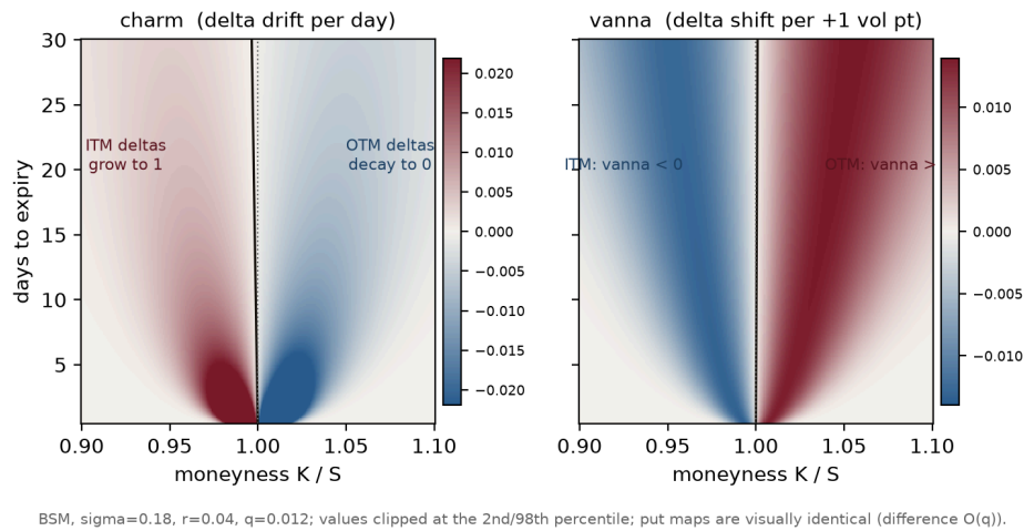
Figure 5. Black-Scholes charm (left, delta drift per calendar day) and vanna (right, delta shift per +1 vol point) across moneyness and time to expiry ( \sigma=0.18 , r=0.04 , q=0.012 ; no market data). The black zero contour sits near d_2 = 0 , just above the money; both greeks change sign across it. Charm is negligible far from expiry — about \pm 0.001 per day at 30 days — and explodes into the last day ( +0.118 for a slightly in-the-money call, -0.125 just out-of-the-money at 1 day) — roughly a hundred-fold amplification. Vanna is largest just off the money and decays more gently with tenor. Reproduce with figures/fig_charm_vanna_maps.py .
