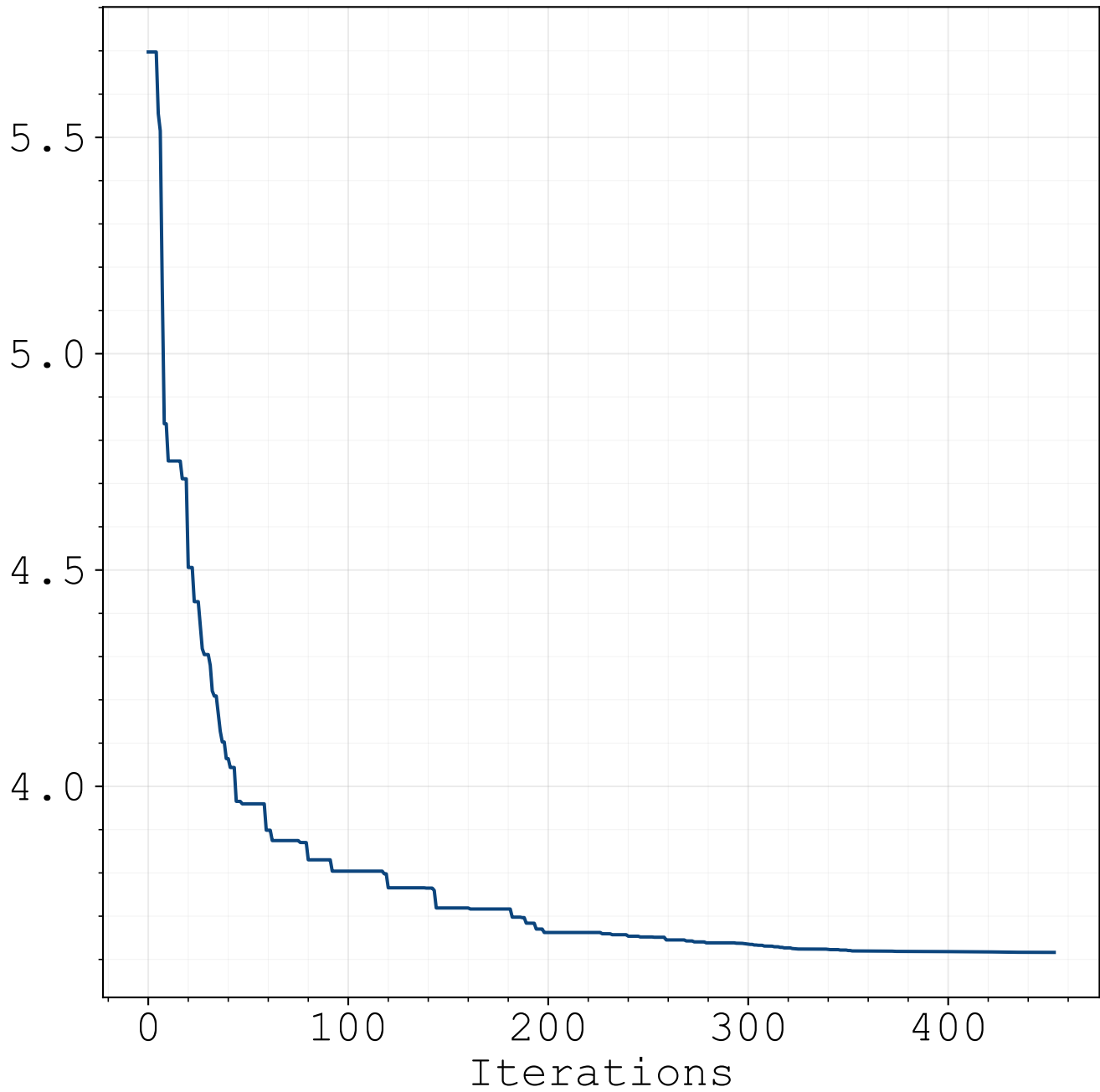
— Cost Function
