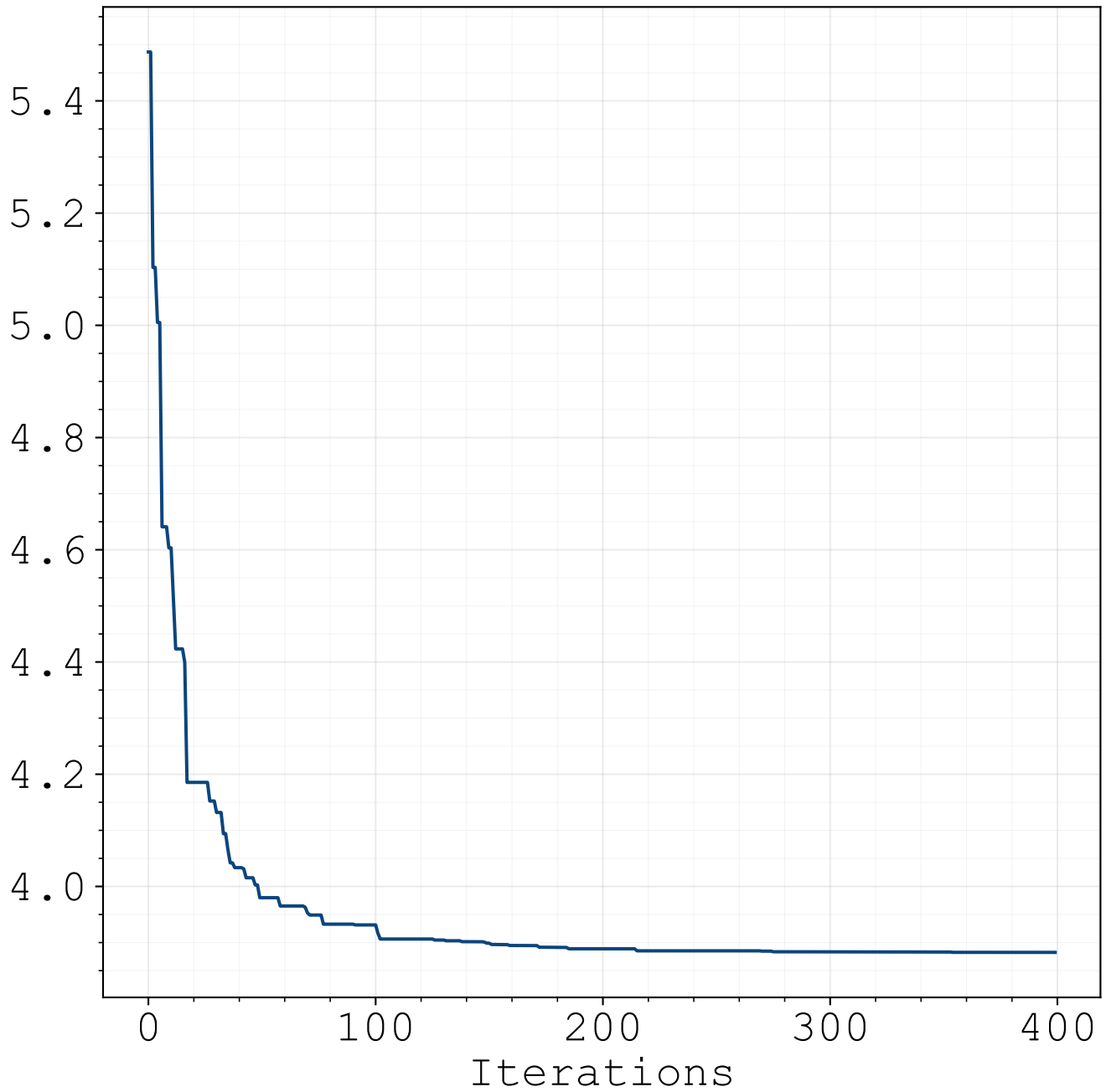
— Cost Function
