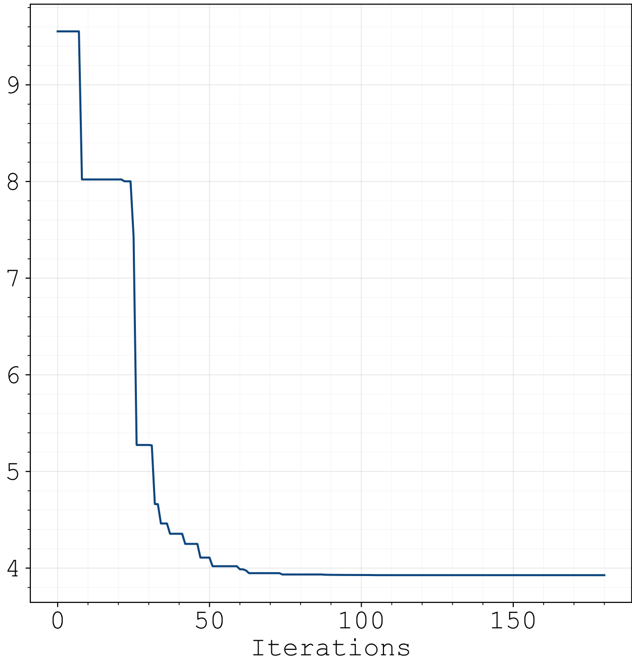
— Cost Function
