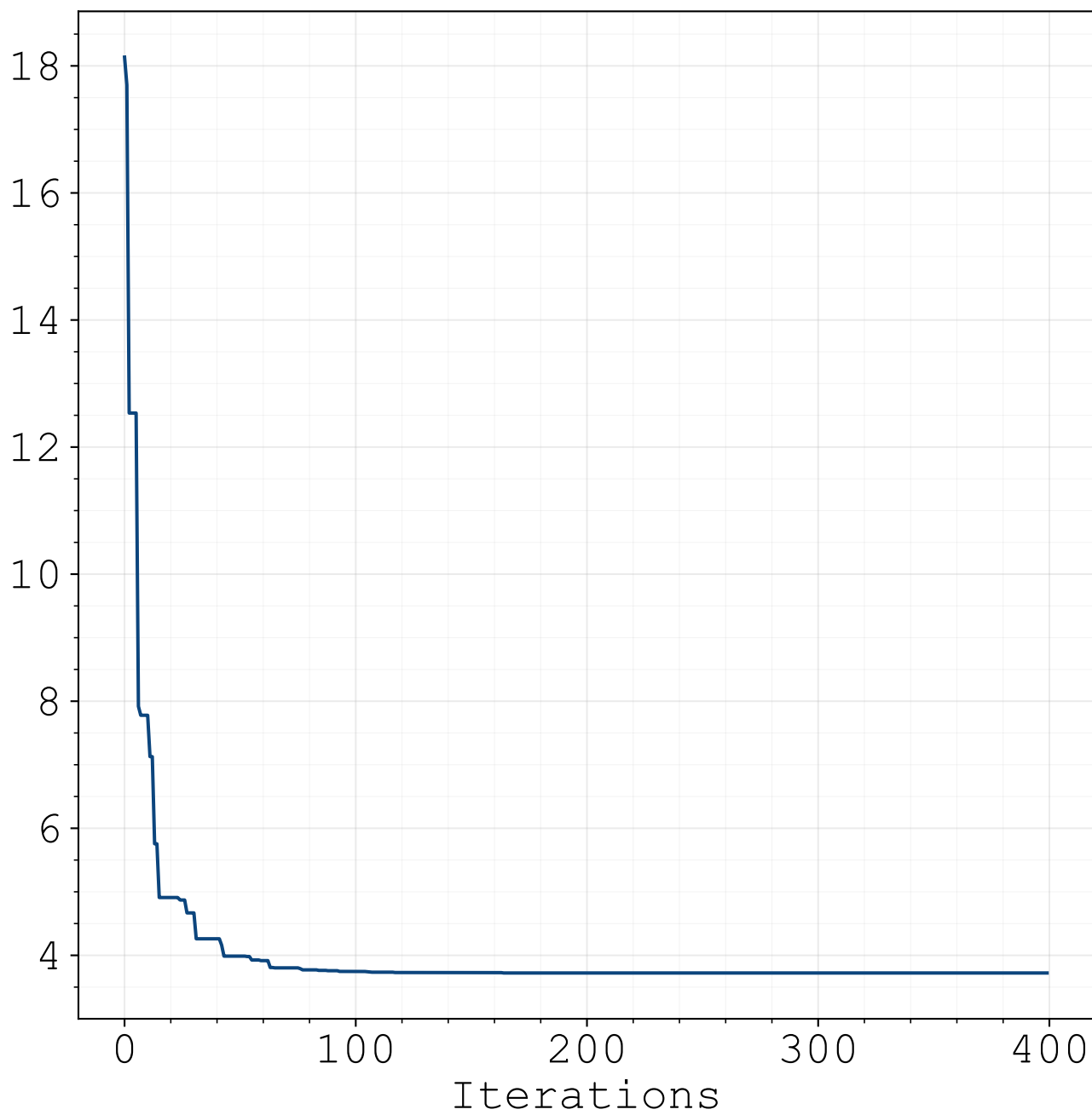
— Cost Function
