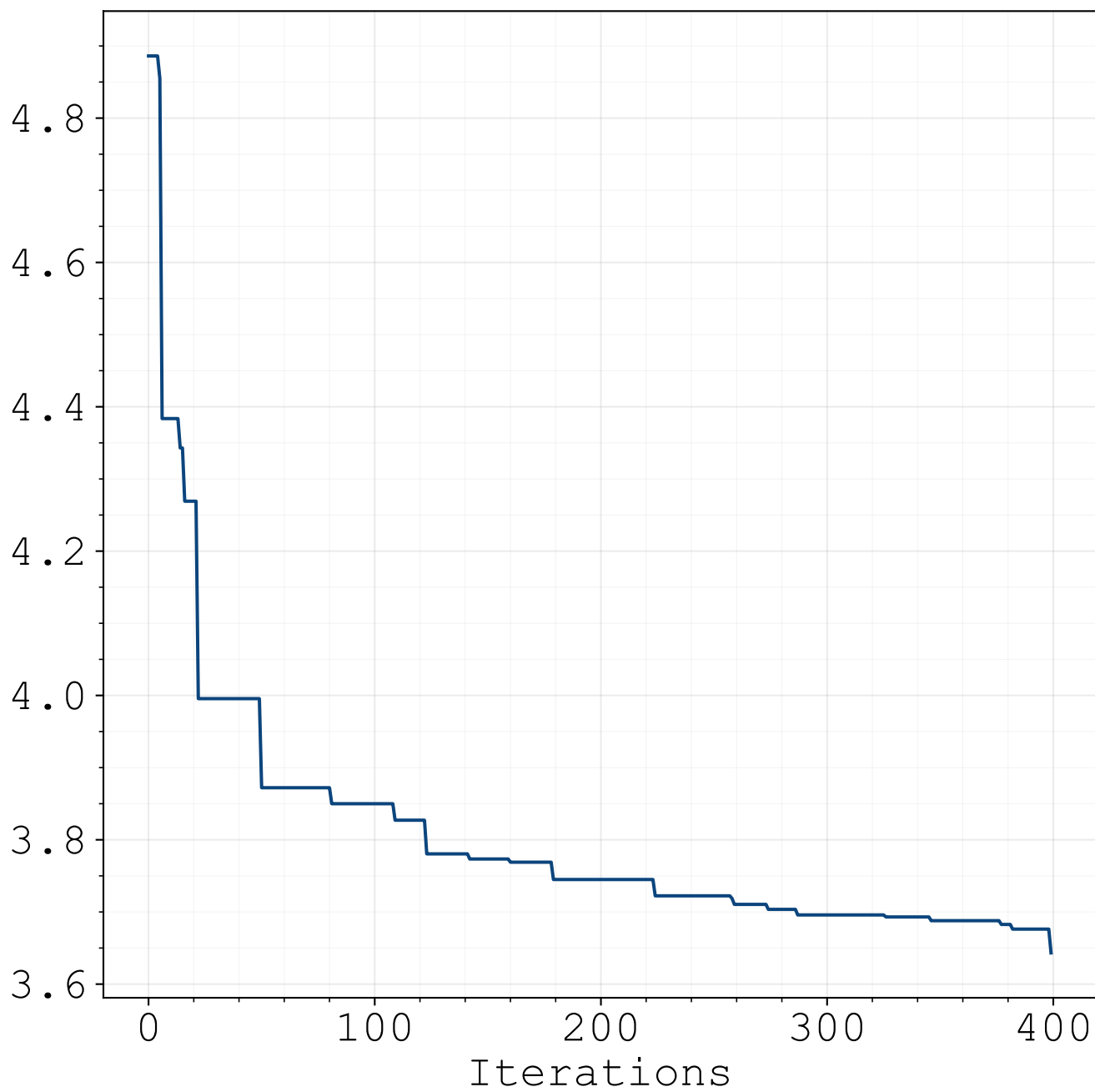
— Cost Function
