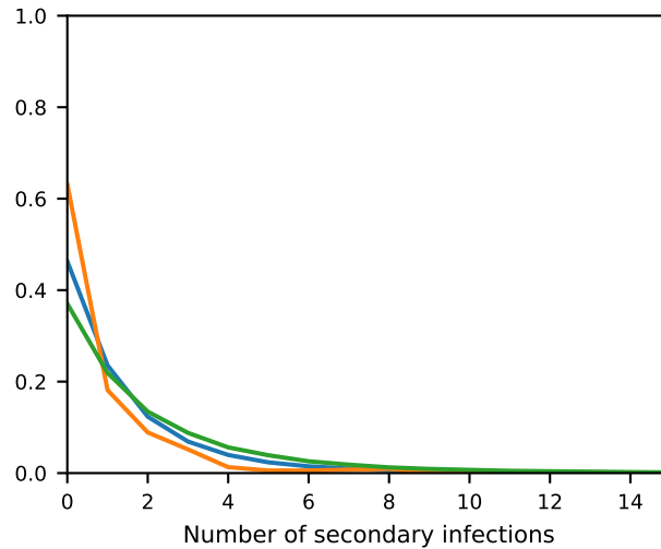
Geometric
