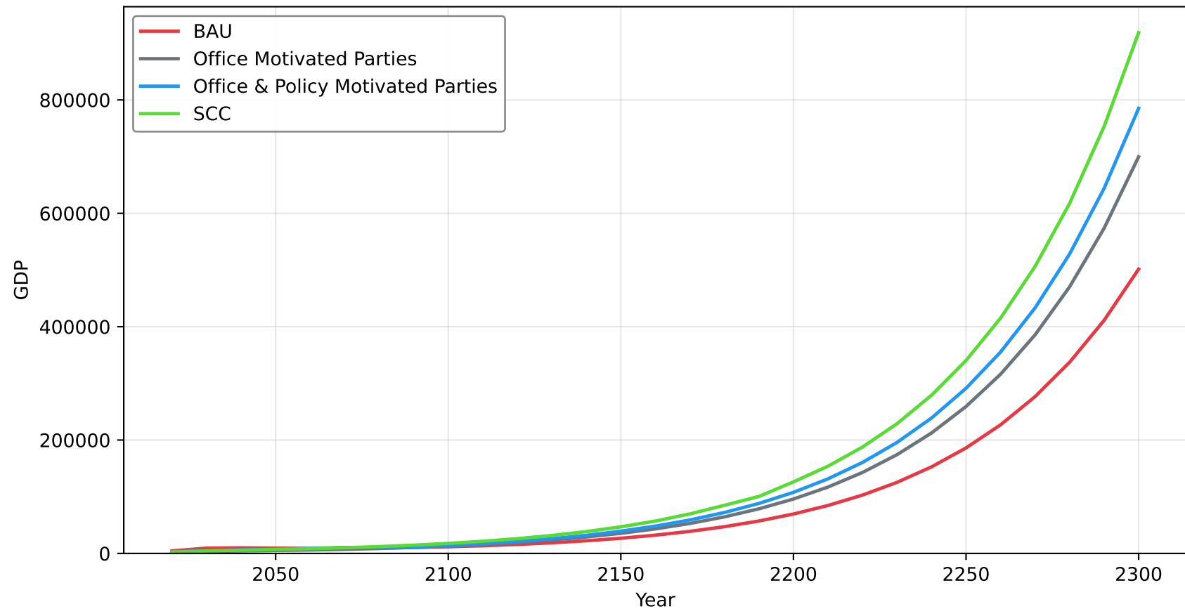
GDP across emission scenarios
