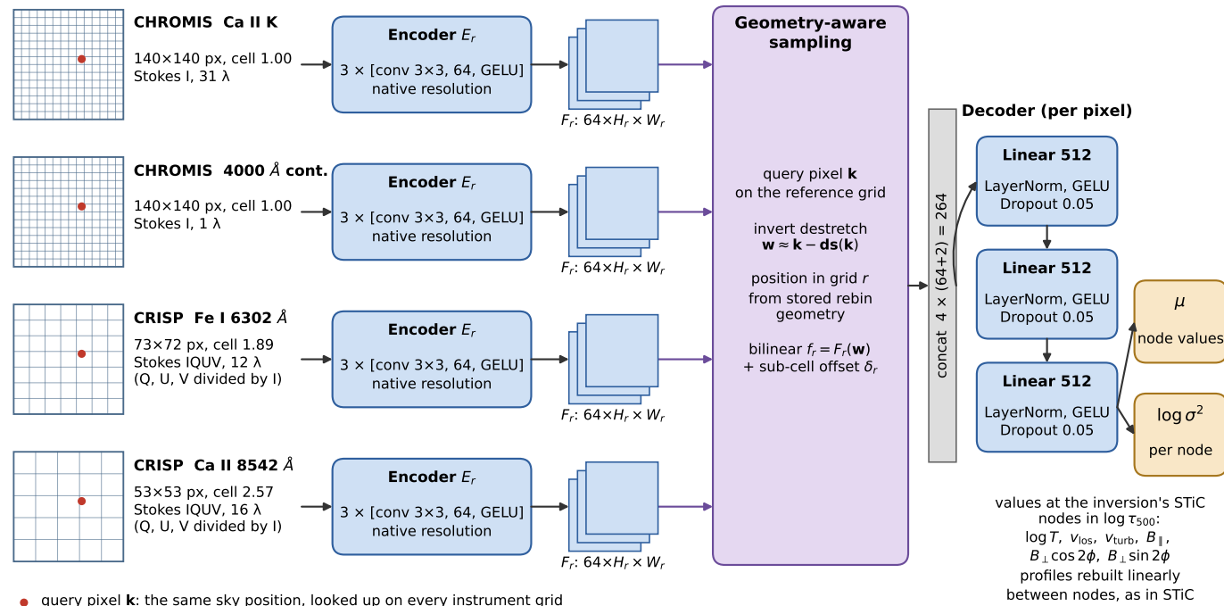
(b) Multi-resolution emulator network (one ensemble member)
