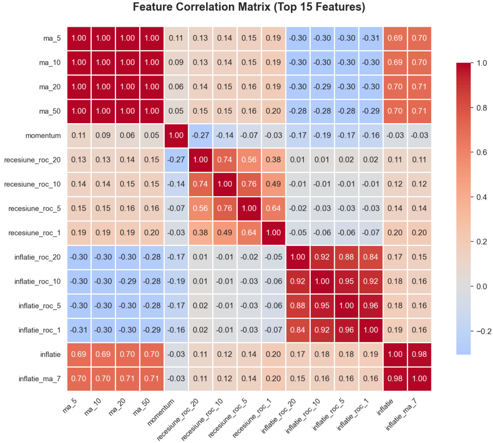
Figure 6: Correlation heatmap of technical indicators
