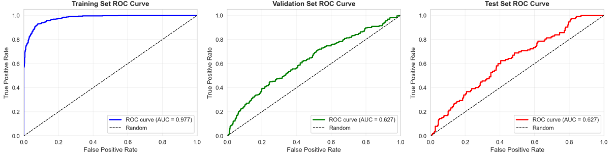
Figure 1: ROC curves for training, validation, and test sets
