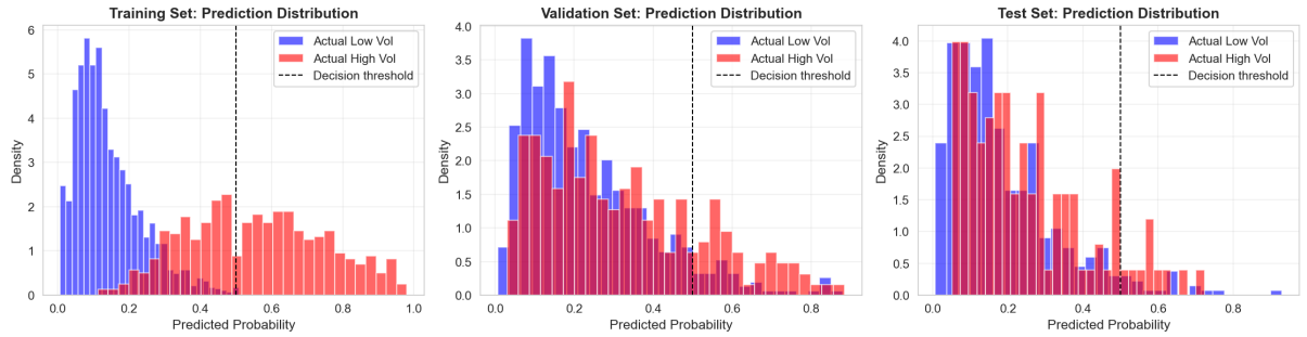
Figure 3: Distribution of predicted probabilities by actual class
