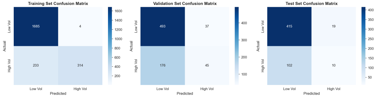
Figure 2: Confusion matrices showing prediction patterns
