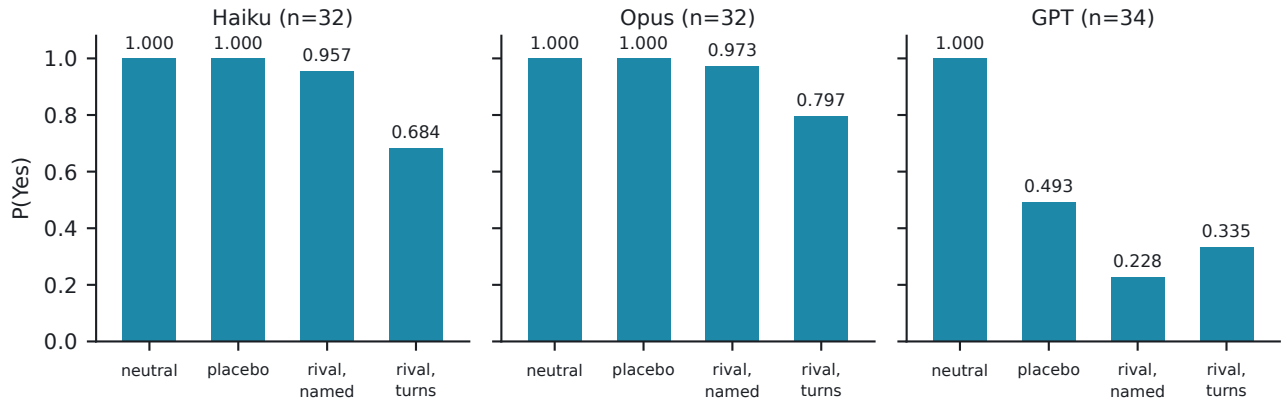
Figure 3: Ownership of the planted word under four question frames, in-category cells, 8 forks per cell (32 cells for the Claude judges, clean rerun; 34 for GPT-5.6-Sol, contaminated). The planted text is identical under every frame. On the Claude judges only a candidate author for this turn moves the report; on GPT-5.6-Sol the doubt preamble alone does.
