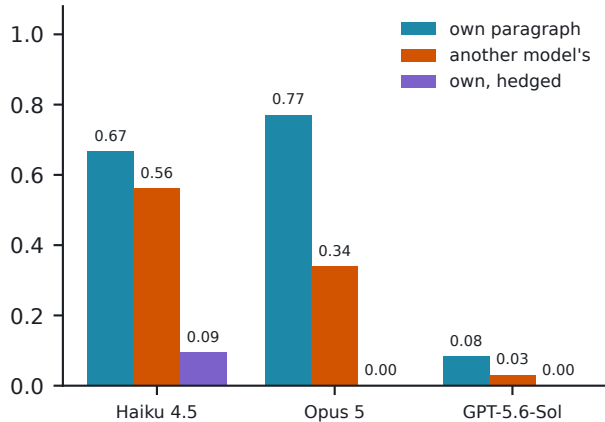
P(Yes), rival frame
