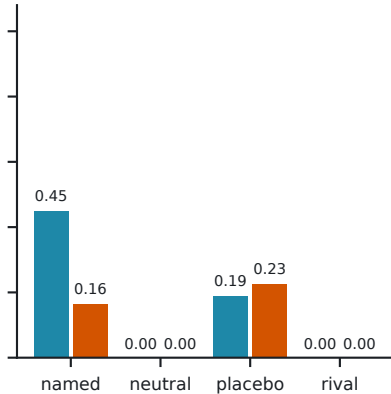
Qwen2.5-3B
