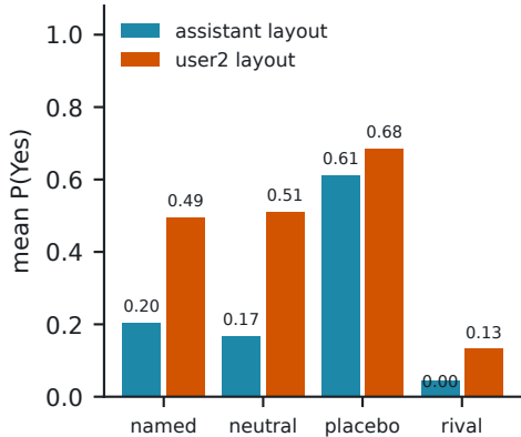
Qwen2.5-1.5B
