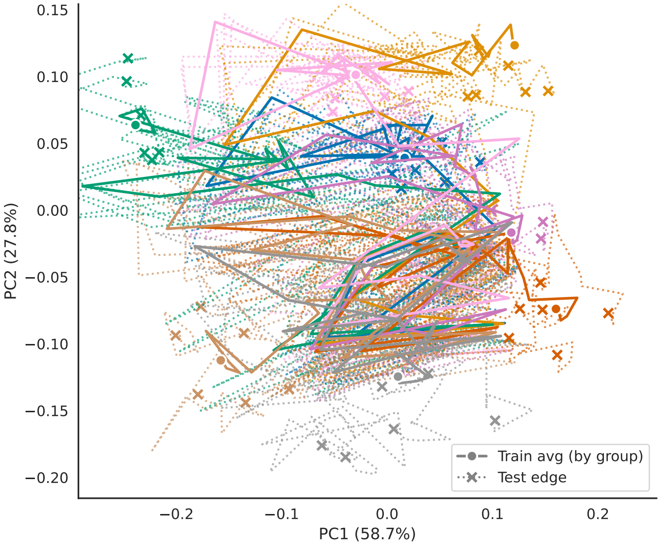
Residual PCA trails (repeat 0)
