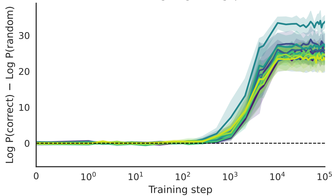
Test-edge log-odds gap
