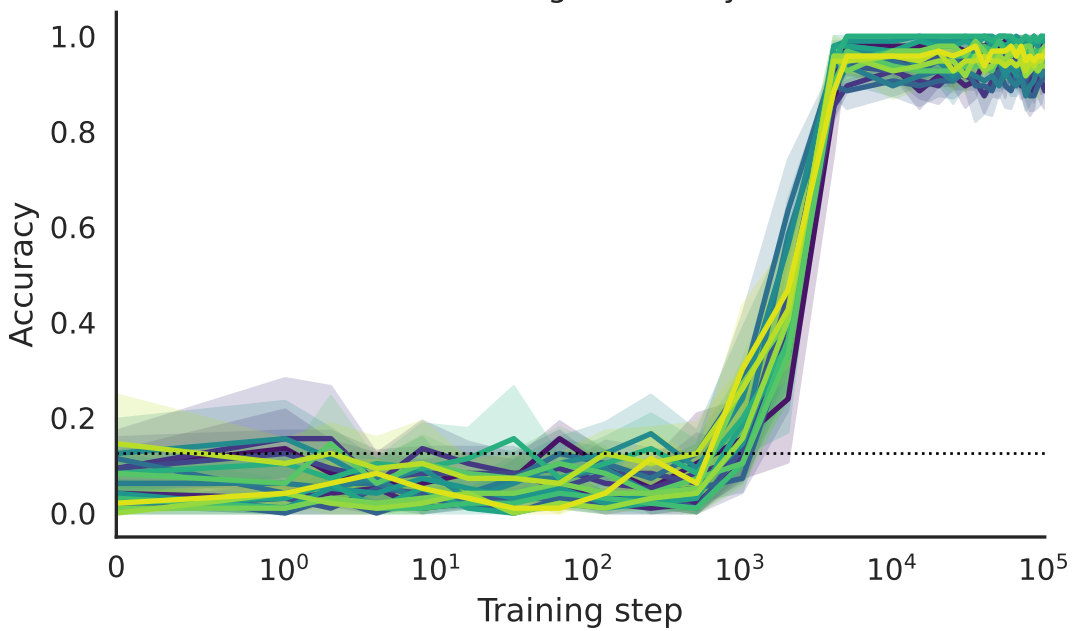
Test-edge accuracy
