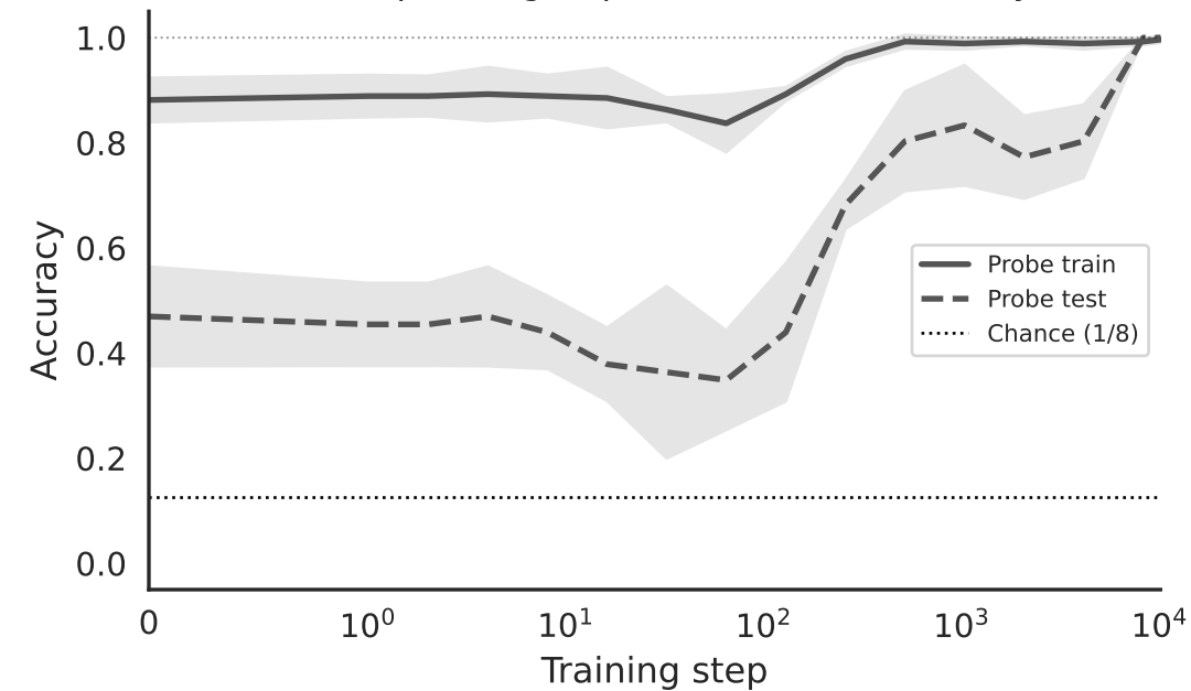
Linear probe: group classification accuracy
